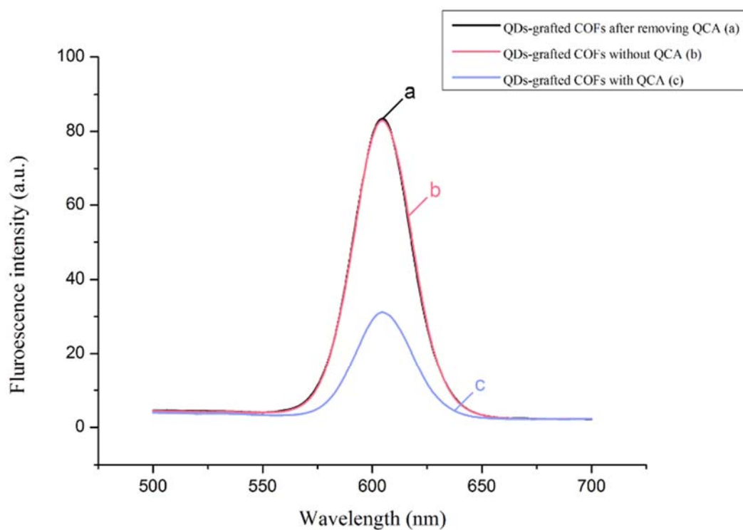
Figure S1. Fluorescence spectra of (a) QDs-grafted COFs after removing QCA, (b) QDs-grafted COFs without QCA, (c) QDs-grafted COFs with QCA.
