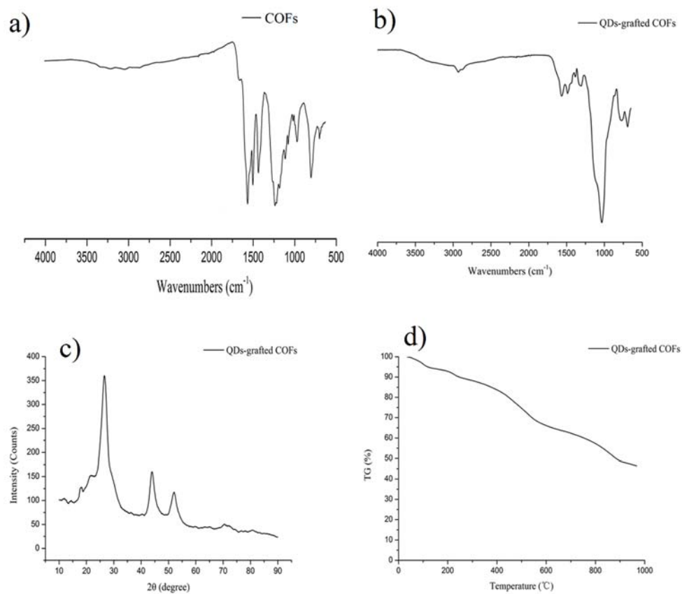
Figure S2. (a) FT-IR spectrum of COFs, (b) FT-IR spectrum of QDs-grafted COFs, (c) XRD spectrum of QDs-grafted COFs, (d) TGA plot of QDs-grafted COFs.
