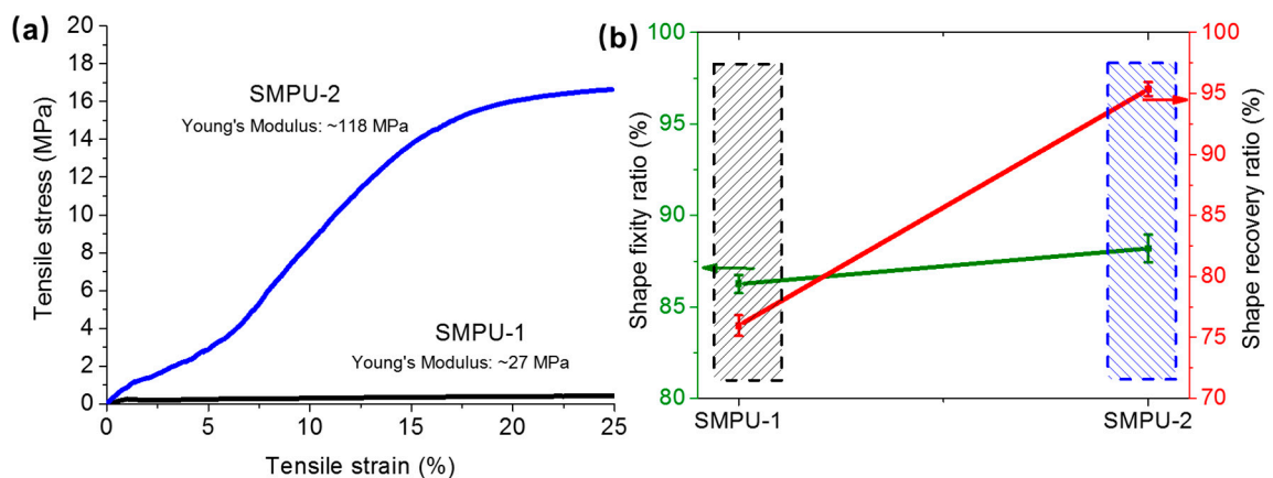
Figure S1. Mechanical (a) and memory properties (b) of the pristine SMPUs
