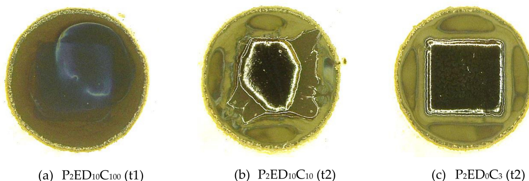
Figure 6. Criteria used in the quality evaluation of the photo-resins corresponding to: (a) 0, (b) 0.5, and (c) 1.0 values.
