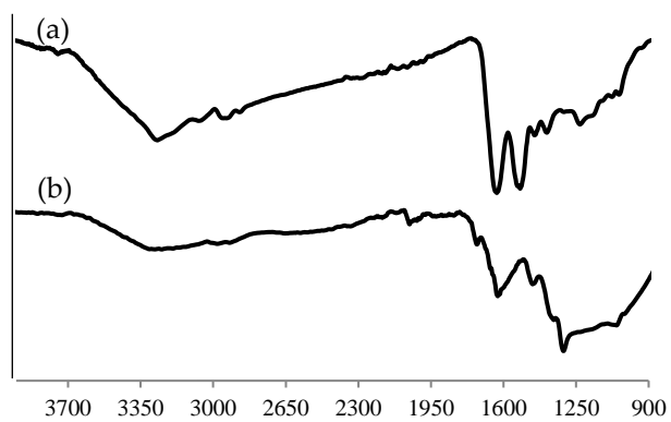
Figure S3. ATR spectra of: (a) keratin, (b) melanin.
