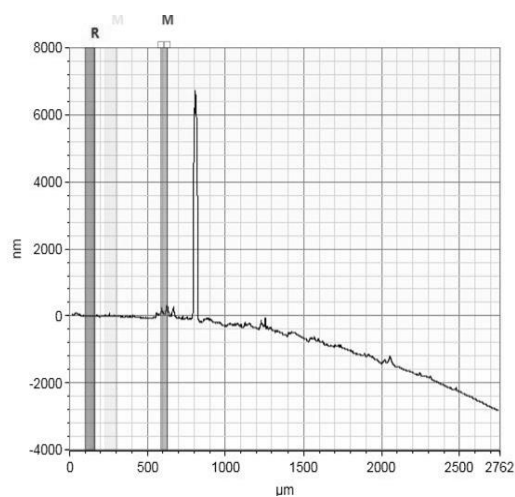
Figure S4: Profiler analysis (Dektak XTTM Stylus Profiler, Bruker, Billerica, MA, USA) for one printed layer of KMI.
