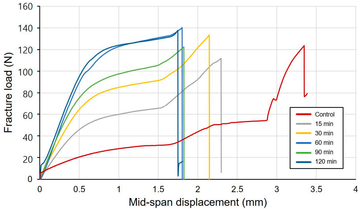
Figure S1. Representative curves of fracture load of the 3D printing resin (DIONavi C&B) used in this study. It can be observed that the fracture load continues to increase as the post-curing time increases, and the shorter the post-curing time, the greater the displacement.
