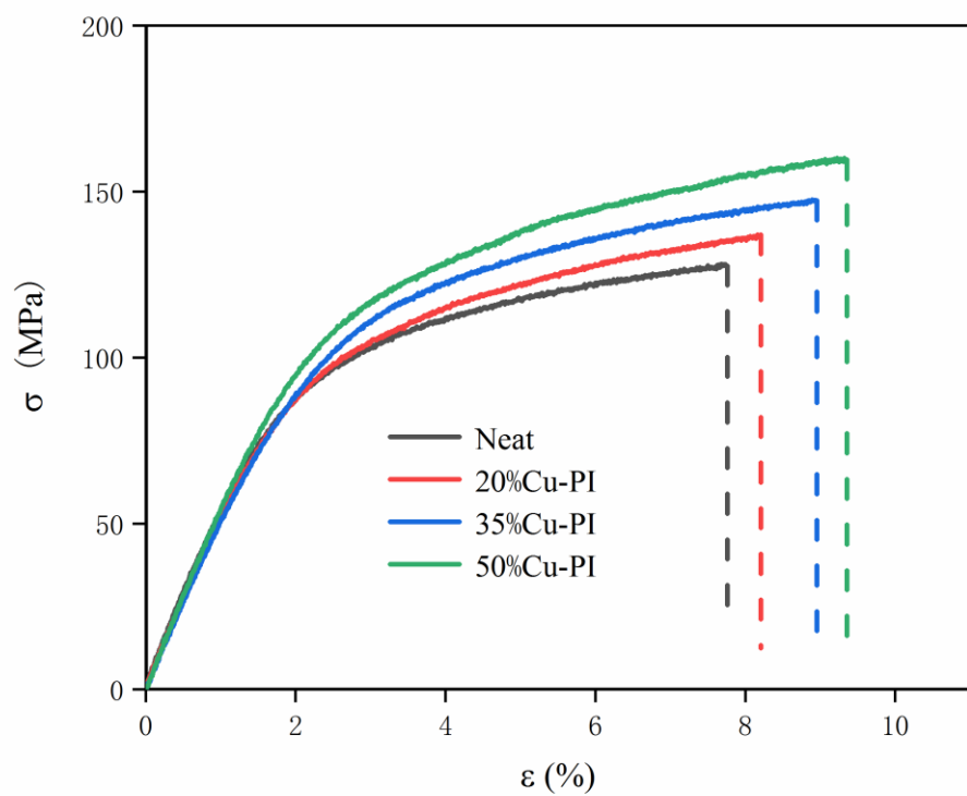
Figure S2. Stress–strain curves of neat PI and Cu-PI films.
