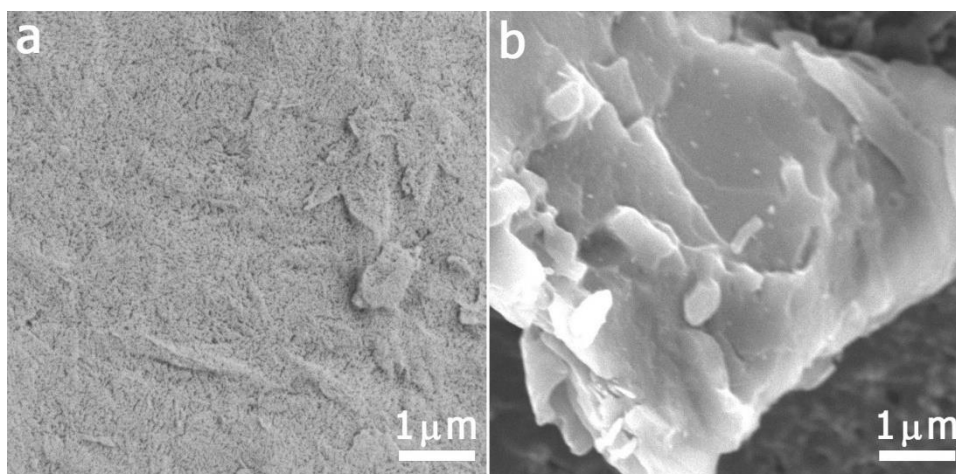
Figure S1. SEM images of cellulose powder before (a) and after (b) pyrolysis.
