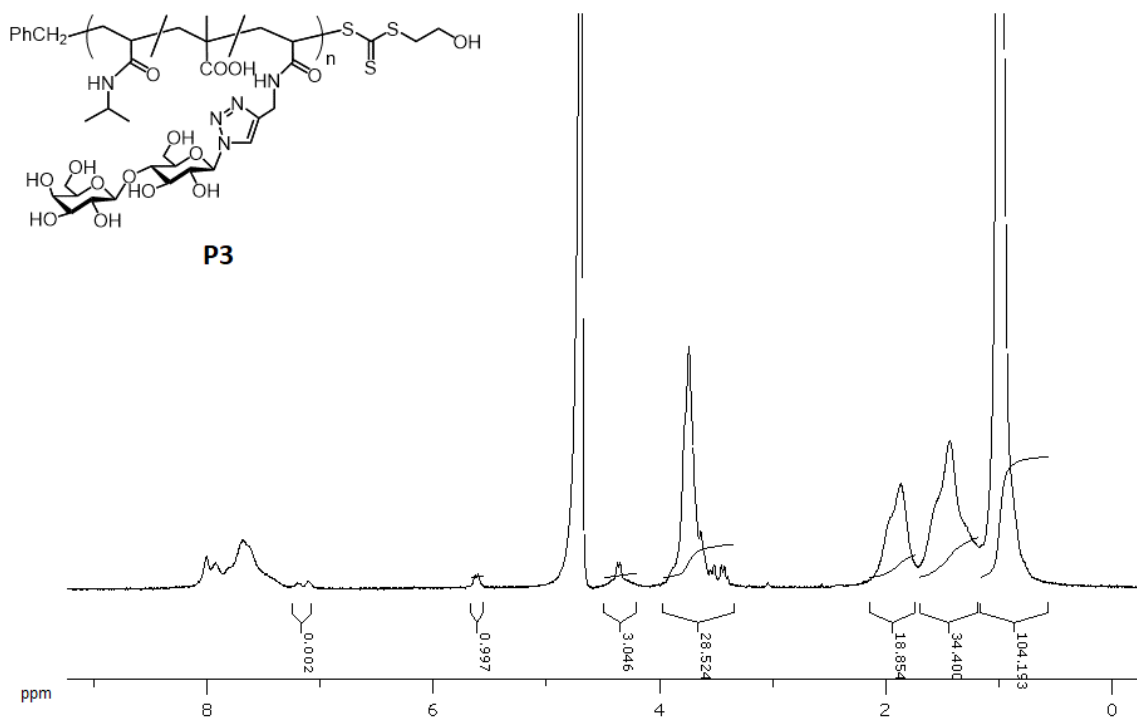
Figure S2 ^1\text{H} NMR spectrum of P3 in \text{D}_2\text{O} .
