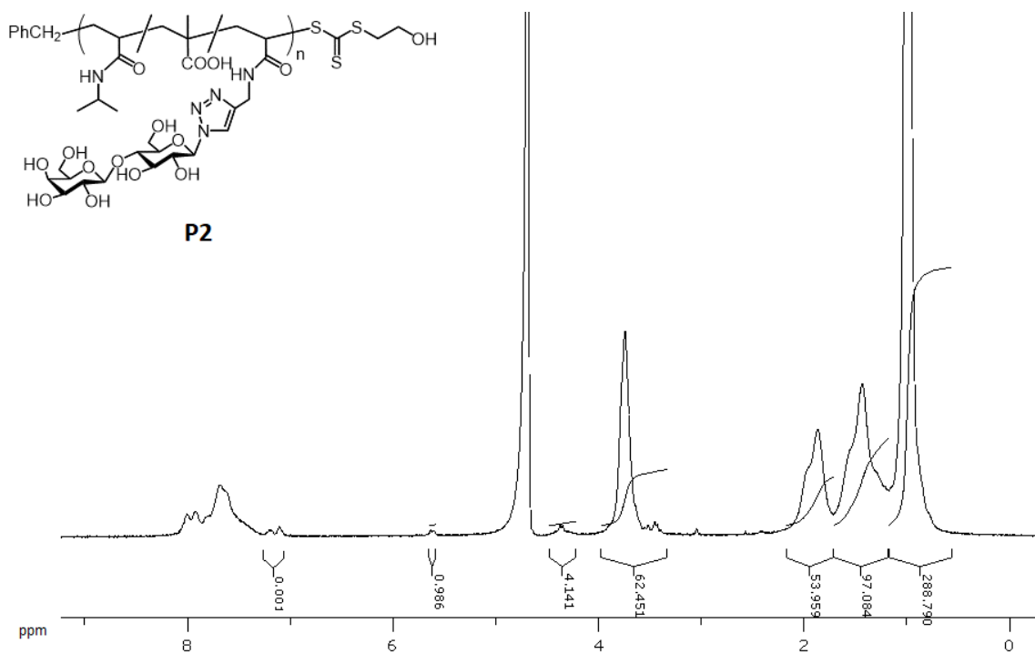
Figure S1 ^1\text{H} NMR spectrum of P2 in \text{D}_2\text{O} .
