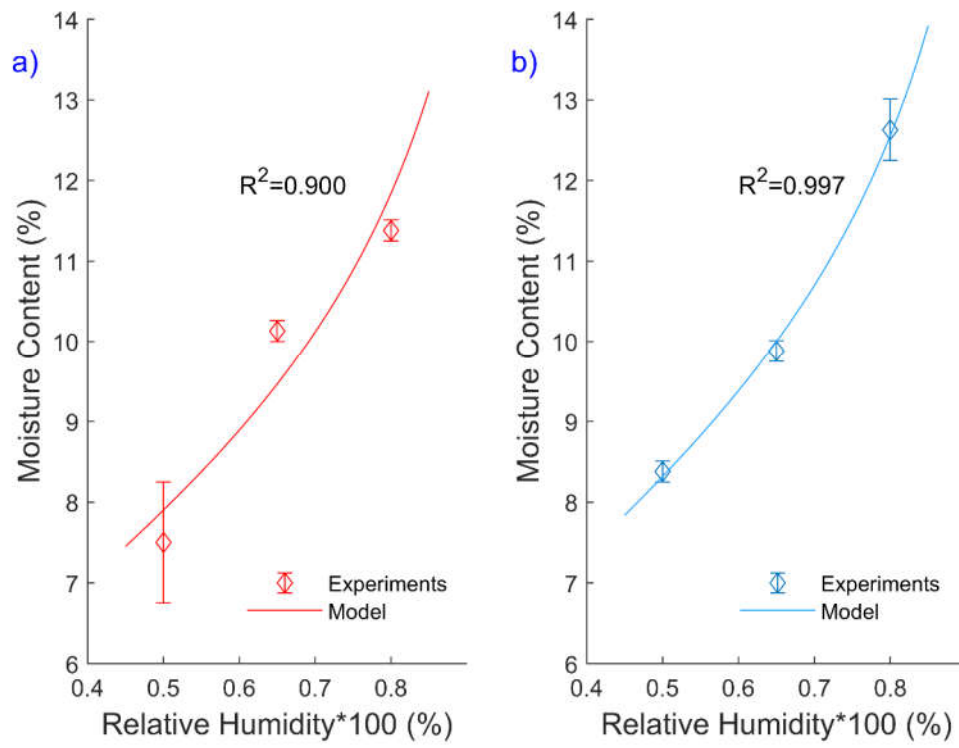
Figure S 2. Moisture uptake at 20°C. Experimental results versus Oswin model for (a) brown and (b) white pellets.
