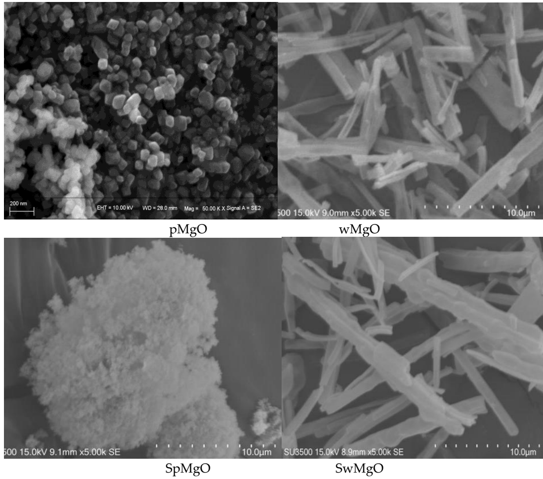
Figure 1. The SEM graphs of pMgO, wMgO, steaic acid modified pMgO and wMgO.
