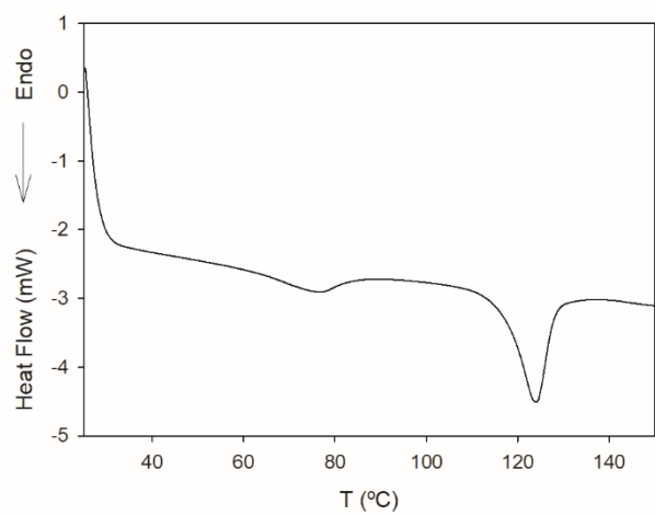
Figure S2: Heat flow curve (1 st heating cycle) of PEU.
