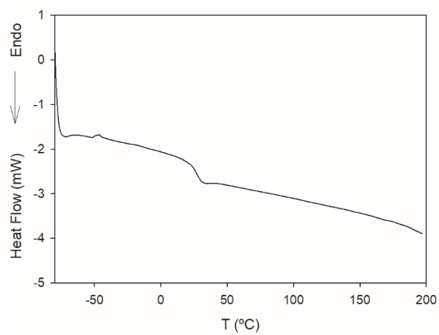
Figure S1: Heat flow curve (2 nd heating cycle) of PEU.
