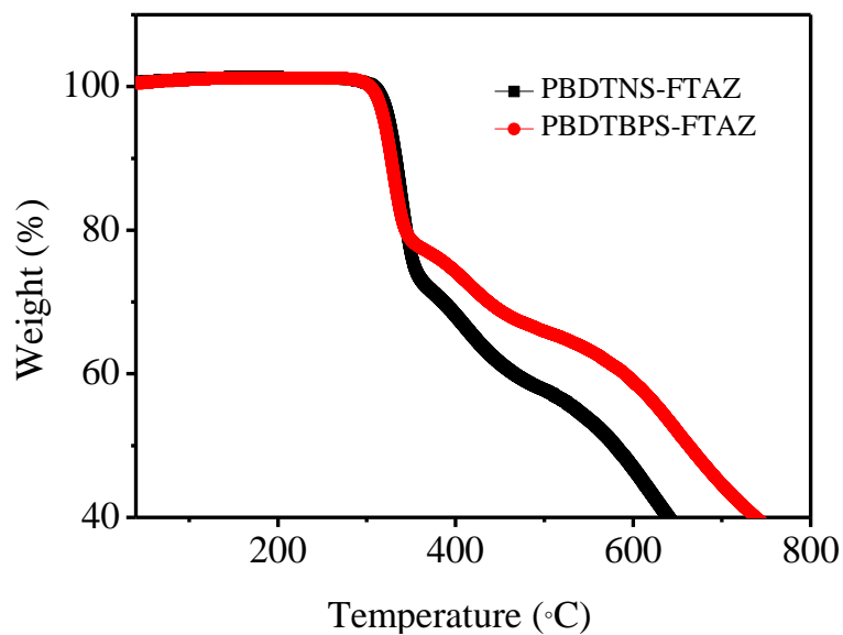
Figure S1. TGA plots of PBDTNS-FTAZ and PBDTBPS-FTAZ.
