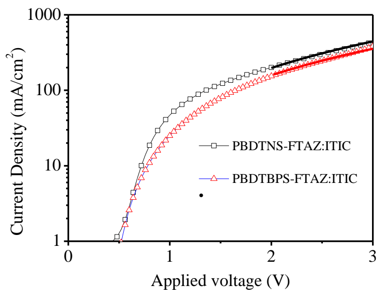
Figure S2. J-V curves of vertical diodes with the device structures of ITO/PEDOT:PSS/polymer:ITIC/Au for hole only devices.
