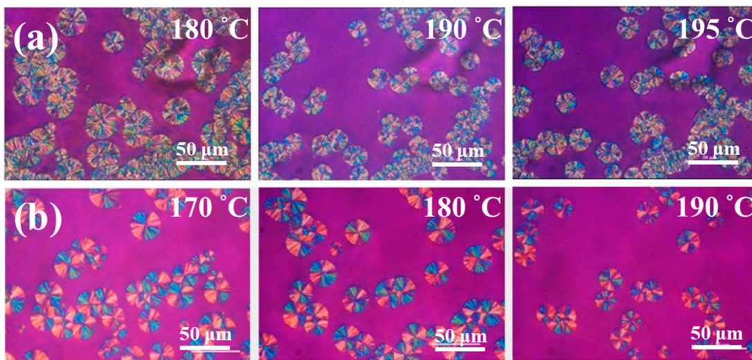
10 Figure S2. PLM image of PBT-co-PTMEG at the selected temperature (a) PBT-co-PTMEG-20 (b) 11 PBT-co-PTMEG-30. 12
