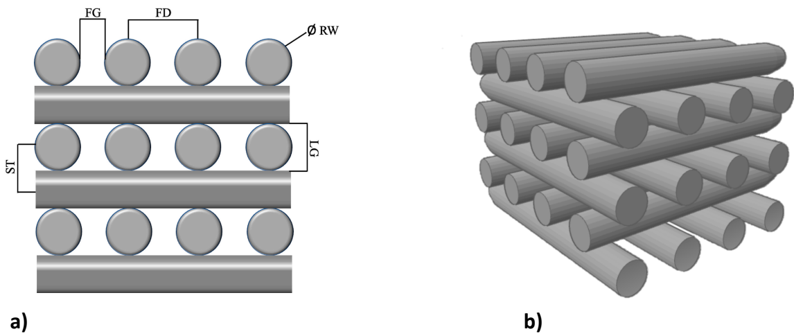
Figure S1. (a) Schematic representation of a cross section viewed in the XZ plane of the building process (RW: road width or filament diameter; FG: filament gap; ST: slice thickness; LG: layer gap; FD: filament distance); (b) 3D illustration of the additive manufactured scaffolds characterized by a 0°/90° lay-down pattern.
