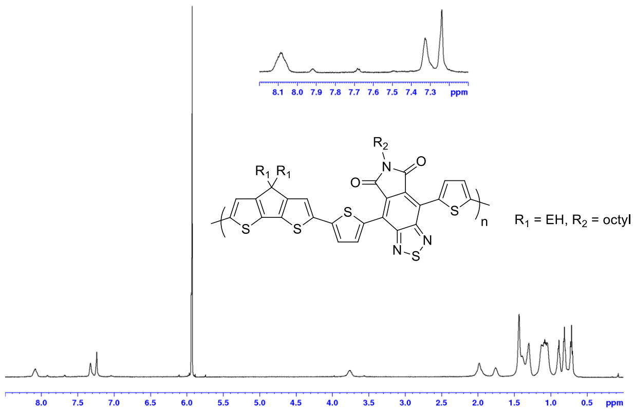
Figure S4. ^1\text{H} NMR spectrum of PCPDTDTBTDI-EH, 8 in \text{C}_2\text{D}_2\text{Cl}_4 at 100\text{ }^\circ\text{C} .
