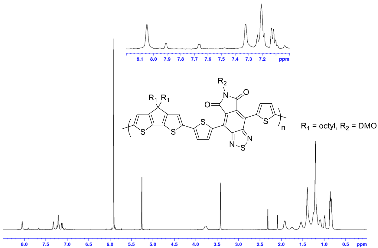
Figure S2. ^1\text{H} NMR spectrum of PCPDTDTBTDI-8, DMO in \text{C}_2\text{D}_2\text{Cl}_4 at 100\text{ }^\circ\text{C} .
