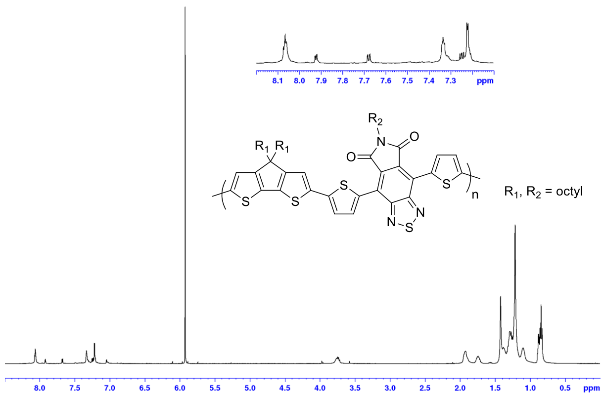
Figure S3. ^1\text{H} NMR spectrum of PCPDTDTBTDI-8, 8 in \text{C}_2\text{D}_2\text{Cl}_4 at 100\text{ }^\circ\text{C} .
