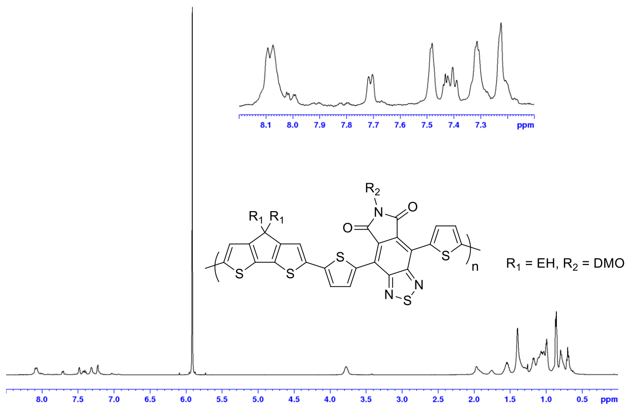
Figure S1. ^1\text{H} NMR spectrum of PCPDTDTBTDI-EH, DMO in \text{C}_2\text{D}_2\text{Cl}_4 at 100\text{ }^\circ\text{C} .
