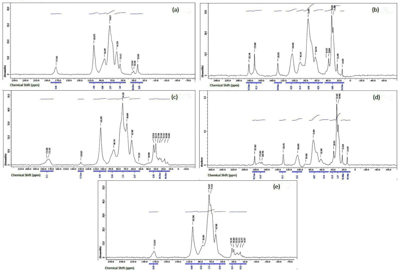
Figure 5. ^{13}\text{C} solid-state NMR spectra of commercially available BG (a), BG obtained from K. marxianus TISTR 5925 by alkaline (b) and enzymatic recovery (c), BG obtained from S. cerevisiae Kyokai NO. 9 by alkaline (d) and enzymatic (e) recovery.
