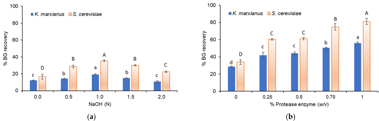
Figure 2. BG recovery by alkaline (a) and enzyme (b) methods using cells of K. marxianus TISTR 5925 and S. cerevisiae Kyokai NO. 9 as raw materials. Different letters a–d and A–D indicate statistically significant differences ( p < 0.05 ) according to Duncan's multiple range test. Error bars show mean \pm SD ( n = 3 ).
