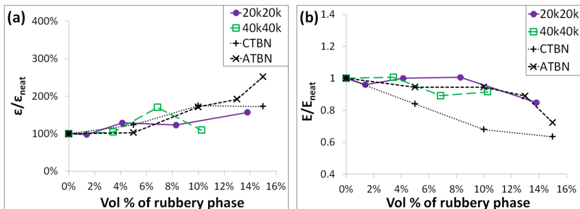
Figure 11. (a) Comparison of the improvement in the strain-to-break vs. the volumetric loading of the rubbery phase between the rubbery copolymer grafted SiO 2 /epoxy nanocomposites and conventional rubber (CTBN and ATBN) filled epoxy composites; (b) Comparison of the Young's modulus vs. the volumetric loading of the rubbery phase between the rubbery copolymer grafted SiO 2 /epoxy nanocomposites and conventional rubber (CTBN and ATBN) filled epoxy composites [29].
