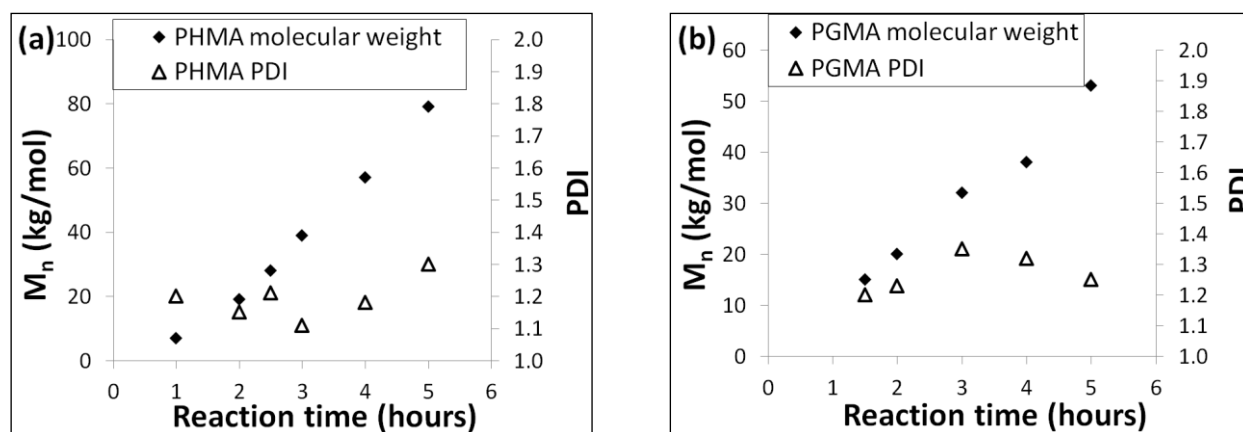
Figure 2. Plots showing the dependence of molecular weight and PDI on reaction time for the RAFT polymerization of HMA (a) and GMA (b) (5 M in THF) at 60 °C with AIBN as initiator ( 1.5 \times 10^{-5} M) mediated with RAFT agent anchored silica nanoparticles ( 1.5 \times 10^{-4} M; 0.61 chains/nm 2 ). The gel permeation chromatography (GPC) system was calibrated with poly(methyl methacrylate) standards.
