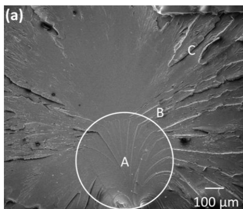
Figure 12. Scanning Electron Micrographs showing the tensile fracture surfaces of (a) the neat epoxy; (b) 0.3 vol% 20k20k-SiO 2 nanocomposites; (c) 1 vol% 20k20k-SiO 2 nanocomposites; (d) 0.1 vol% 40k40k-SiO 2 nanocomposites; and (e) 0.2 vol% of 40k40k-SiO 2 nanocomposites. "A": mirror zone, "B": mist zone and "C": hackle zone.
