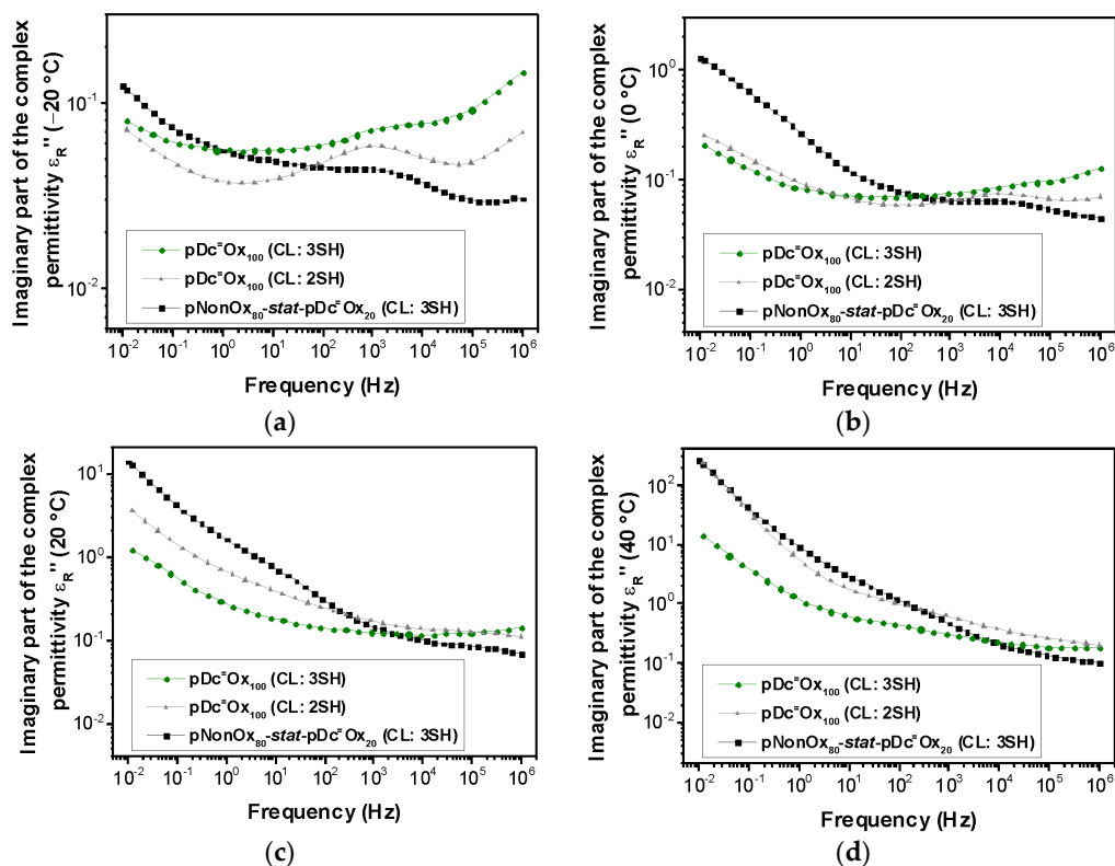
Figure 2. Frequency-dependent imaginary part of the complex permittivity of pNonOx 80 -stat-pDc = Ox 20 (CL:3SH), pDc = Ox 100 (CL:2SH), and pDc = Ox 100 (CL:3SH) at -20 °C (a), 0 °C (b), 20 °C (c) and 40 °C (d).
