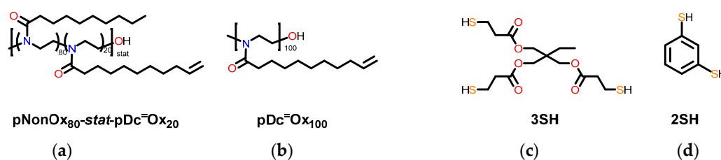
Scheme 3. Reactants for the thiol-ene reactions used in this study: (co)poly(2-oxazoline)s as ene components (a and b) and di- and trimercapto compounds as thiol components (c and d).
