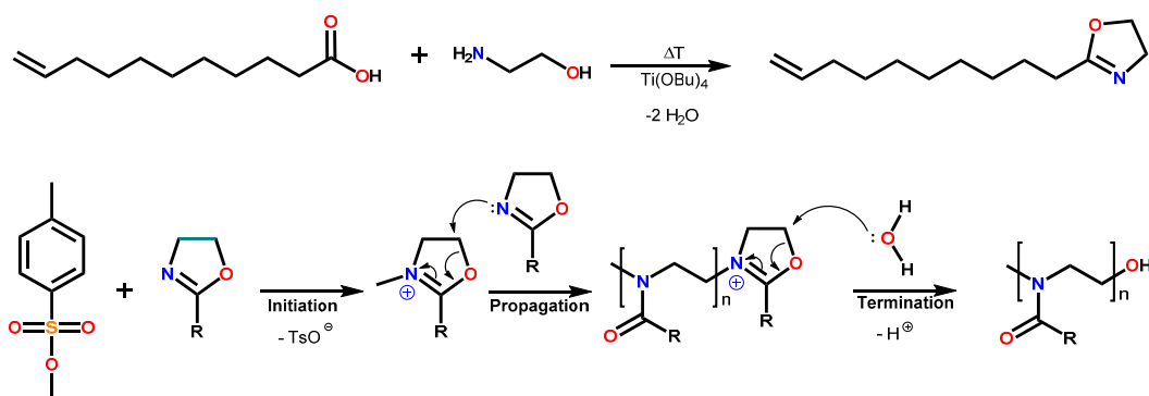
Scheme 1. Schematic representations of the synthesis of 2-oxazoline monomers from carboxylic acids ( top ) and the cationic ring-opening polymerization of 2-oxazolines ( bottom ).
