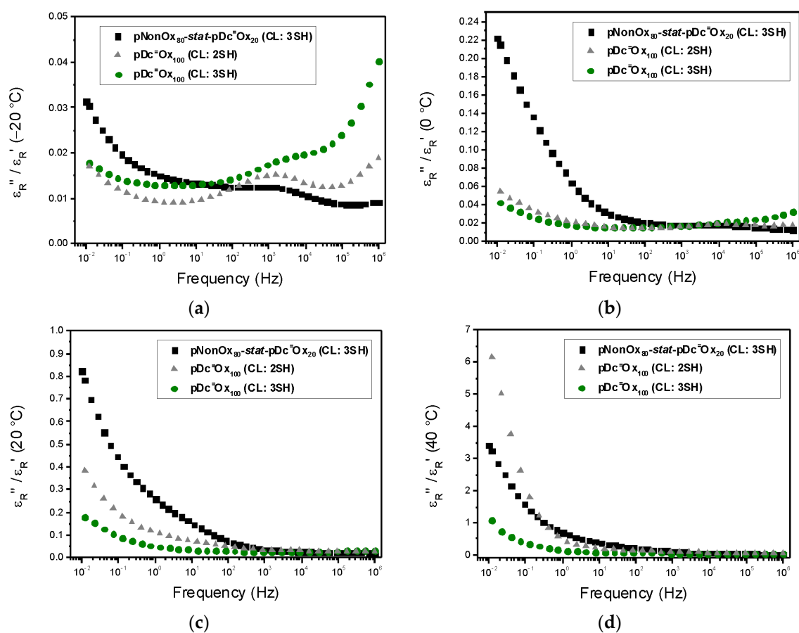
Figure 3. Frequency-dependent loss factors of \text{pNonOx}_{80}\text{-stat-pDc}^{\circ}\text{Ox}_{20} (CL:3SH), \text{pDc}^{\circ}\text{Ox}_{100} (CL:2SH), and \text{pDc}^{\circ}\text{Ox}_{100} (CL:3SH) at -20\text{ }^{\circ}\text{C} (a), 0\text{ }^{\circ}\text{C} (b), 20\text{ }^{\circ}\text{C} (c) and 40\text{ }^{\circ}\text{C} (d).
