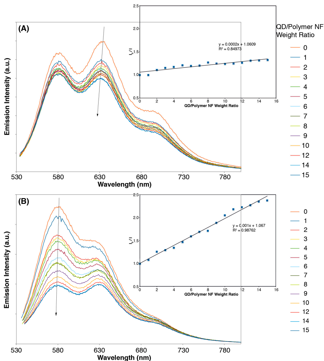
Figure S1. Fluorescence spectra of P3HT NFs (A) and BCP3 NFs (B) in the presence of QDs with PDTCL ligands of various weight ratios. Inserts: corresponding Stern-Volmer plots.
