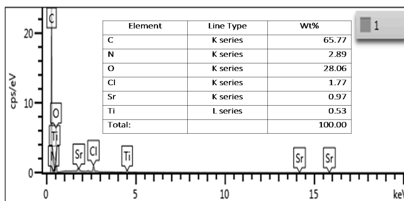
Figure S3. EDX spectrum of GOPSr-2 nanocomposite.
