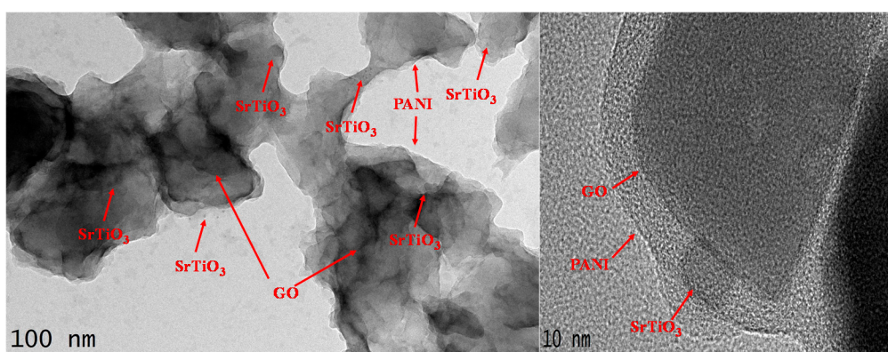
Figure S2. TEM images GOPSr-2 nanocomposite at different magnifications.
