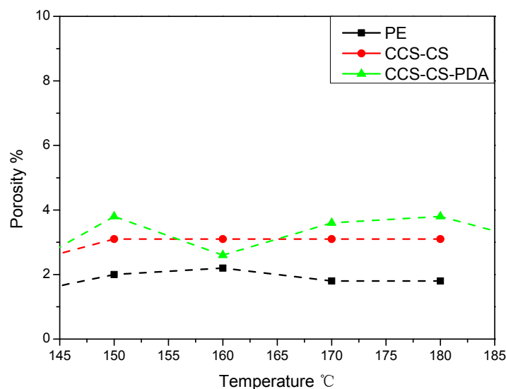
Figure S1. Porosity change with the temperature of the PE separator, CCS-CS and CCS-CS-PDA.
