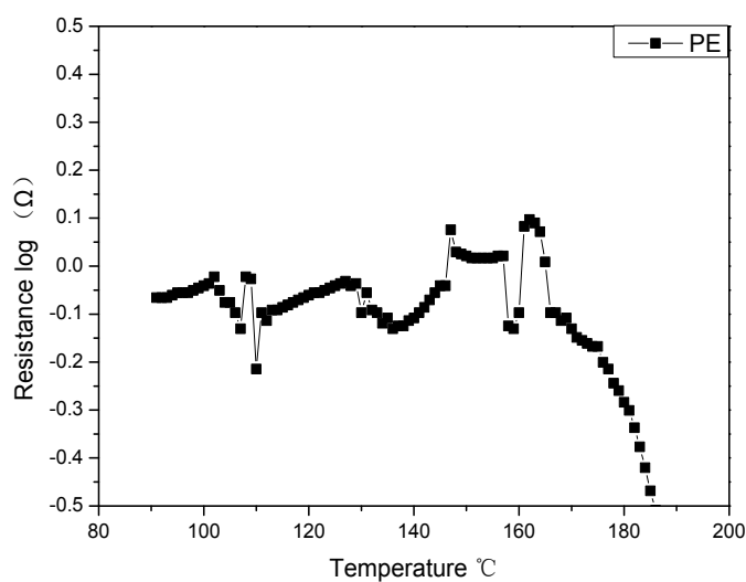
Figure S2. Shutdown behavior of the PE separator.
