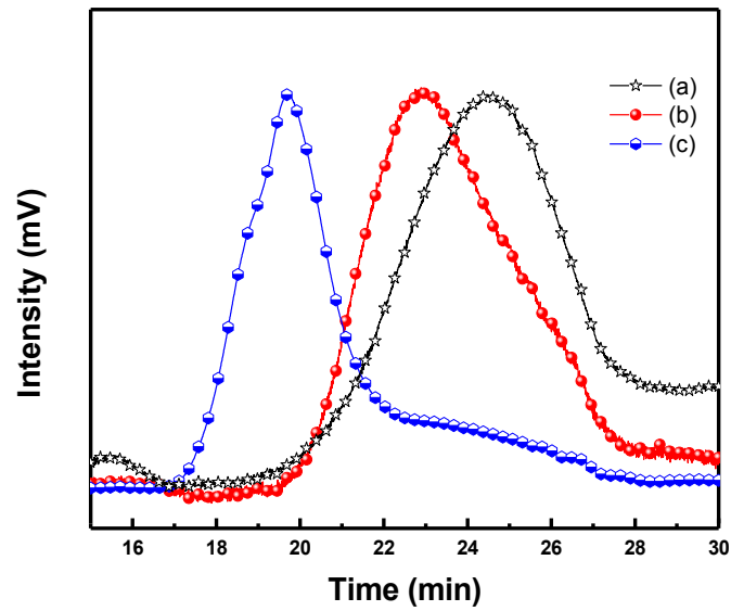
Figure S1. GPC curves of the prepared (a) POF 10 ; (b) POF 10 -b-PDMAEMA 90 and (c) POF 10 -b-PDMAEMA 197 .
