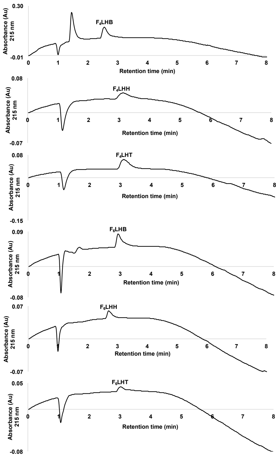
Figure S2. HPLC chromatograph for F 4 LHD and F 6 LHD monomers at day 0.
