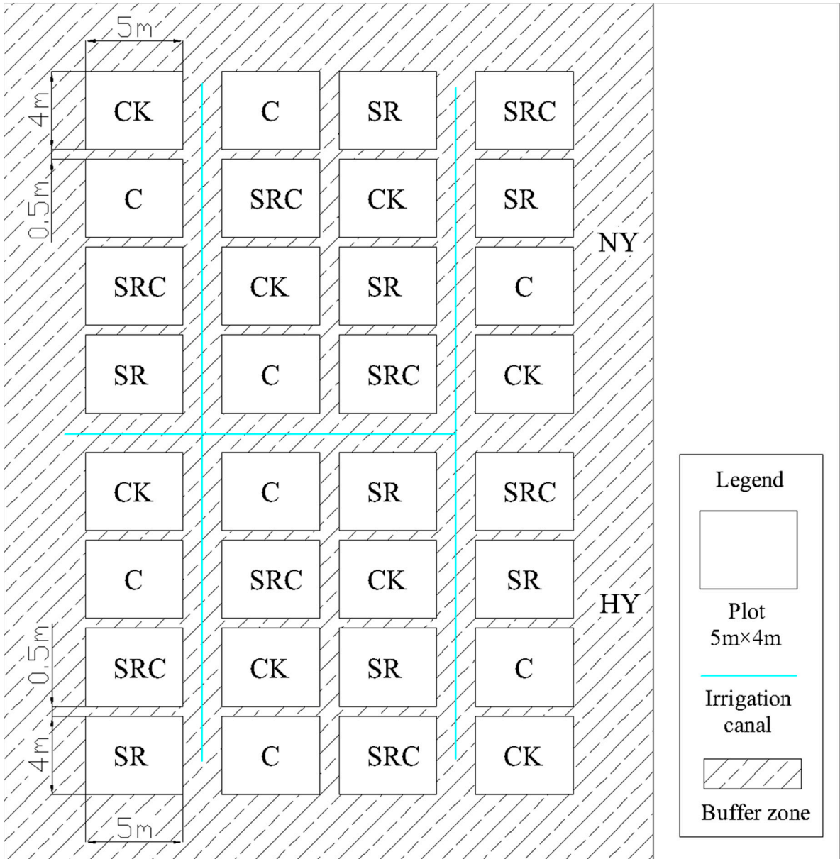
Figure S1. Schematic diagram of the field layout. NY, 90 kg N \text{hm}^{-2} and 45 kg P \text{hm}^{-2} and HY, 270 kg N \text{hm}^{-2} , and 135 kg P \text{hm}^{-2} . CK, sand only; C, sand and biochar; SR, sand and soft rock; SRC, sand, biochar, and soft rock. The blue line indicated the PVC pipe for irrigation, and slash indicated the buffer zone.
