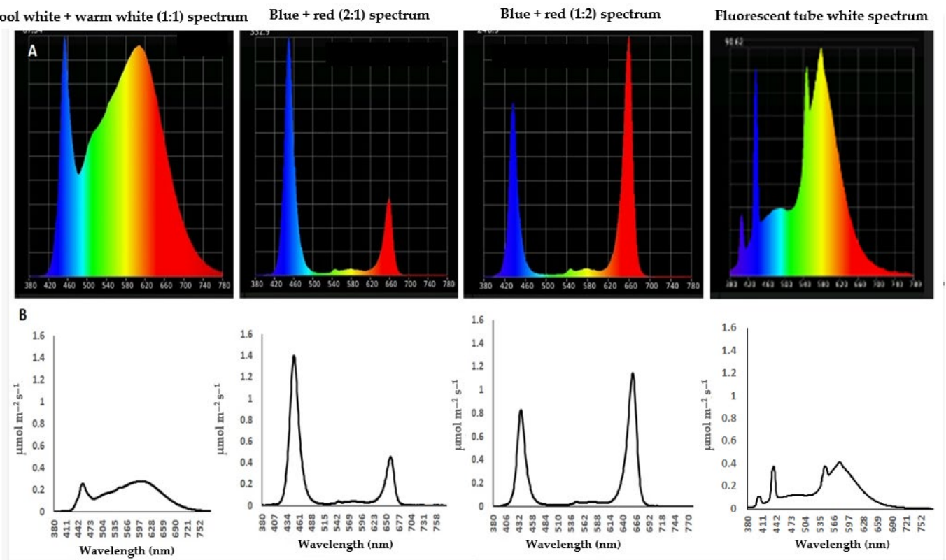
Figure 1. Measured spectra of the light treatments using a UPRtek spectrophotometer. (A) Relative light intensity. (B) Radiant density of the light spectrum intensity.
