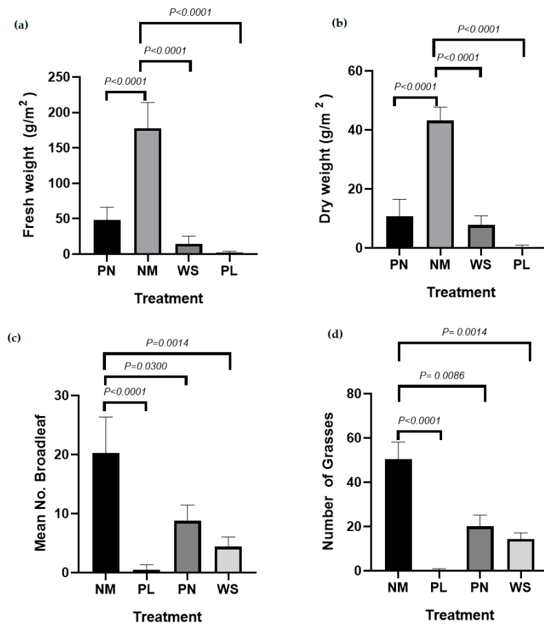
Figure 2. Weed density (Fresh and dry weight) and general weed biomass (number of broadleaf and grasses) reduced significantly in mulch treatments: No mulch (NM), Black Plastic Mulch (PL), Pine Needle Mulch (PN) and Wheat Straw Mulch (WS). (a) Fresh weight of weeds, (b) dry weight of weeds, (c) Number of broadleaf weeds, (d) Number of grassy weeds.
