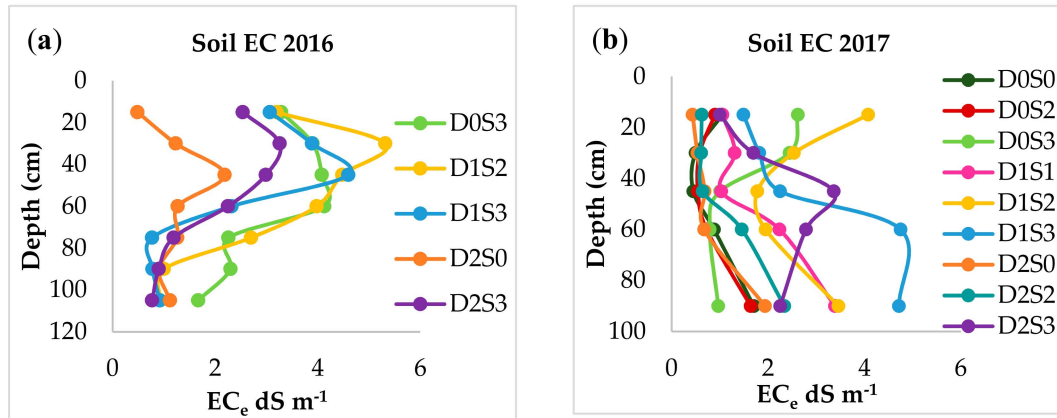
Figure 3. Saturation extract electrical conductivity of select treatments with depth for (a) 2016 and (b) 2017. The designated symbols represent the treatment water applications (D0 = ET_c , D1 = 80% ET_c , D2 = 60% ET_c ), S0 represents irrigation treatments with EC = 0.7 \text{ dS m}^{-1} water, S1 = irrigation with EC = 1.7 \text{ dS m}^{-1} water, S2 = irrigation with EC = 2.7 \text{ dS m}^{-1} water and S3 = irrigation with EC = 3.7 \text{ dS m}^{-1} water.
