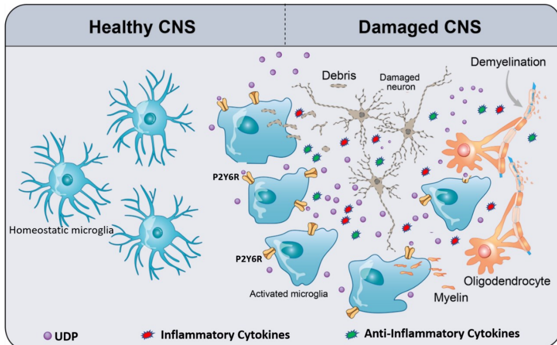
Figure 1. Schematic of UDP/P2Y6R signaling, mediating microglial phagocytosis and chemotaxis. In the healthy CNS, homeostatic microglia (resting microglia) constantly survey and scan the cerebral microenvironment by continuously extending and retracting their ramified processes for the early recognition of damage-associated molecular patterns (DAMPs) such as ATP. Damaged CNS elements (neurons and oligodendrocytes) release or leak ATP/UTP. Furthermore, UTP is easily converted to UDP by ectonucleotidases. UDP acts as an “find-me” signal for P2Y6R. UDP/P2Y6R activates microglia, activated microglia move to the damaged area, and then subsequently recognize UDP as “find-us” signal, attached to the targets, and engulf them. As a result of microglia activation, they release a plethora of inflammatory and anti-inflammatory cytokines depending on the context of the disease. The types and levels of released cytokines differ from a disease to another. The context of a specific disease determines the harmful or the beneficial effects of microglia activation.
