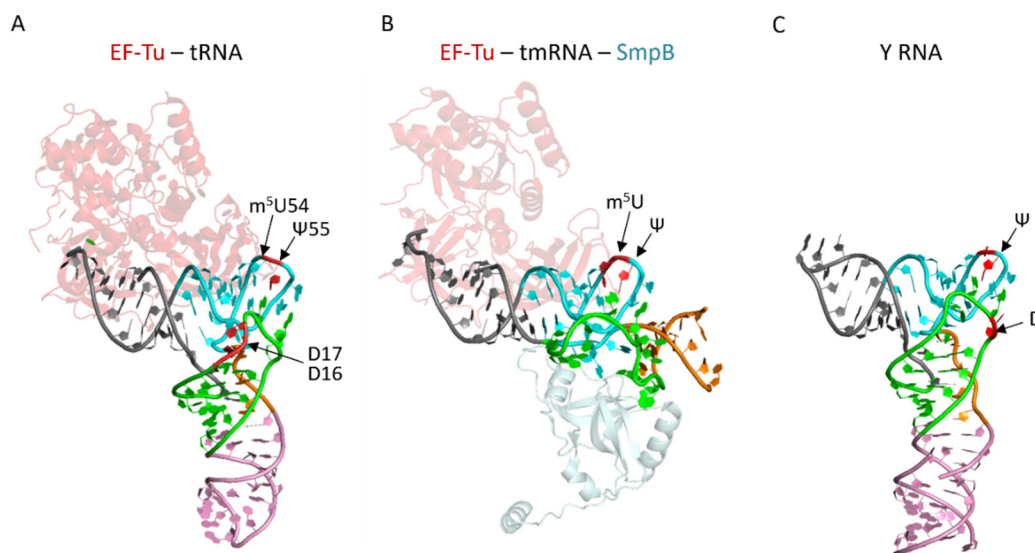
Figure 3. The structures of tmRNA and Y RNA mimic part of the tRNA structure. (A) The structure of EF-Tu-tRNA Phe complex (with GDPNP, GTP analog) from Thermus aquaticus (pdb file 1TTT [189]). Each domain of the tRNA is colored: acceptor arm in grey, TY-arm in light blue, the variable region in orange, the D-arm in green, and the anticodon-arm in pink. EF-Tu structure is represented in light pink. (B) The structure of the tmRNA fragment in complex with EF-Tu (with GDP and kirromycin antibiotic, in light pink) and SmpB (in light grey) from Thermus thermophilus (pdb file 4V8Q [190]). The regions of tmRNA mimicking tRNA are shown with the same color code as for the tRNA. (C) Salmonella Typhimurium Y RNA (YrIA, pdb file 6CU1 [191]). The regions of YrIA mimicking tRNA are shown with the same color code as for the tRNA.
