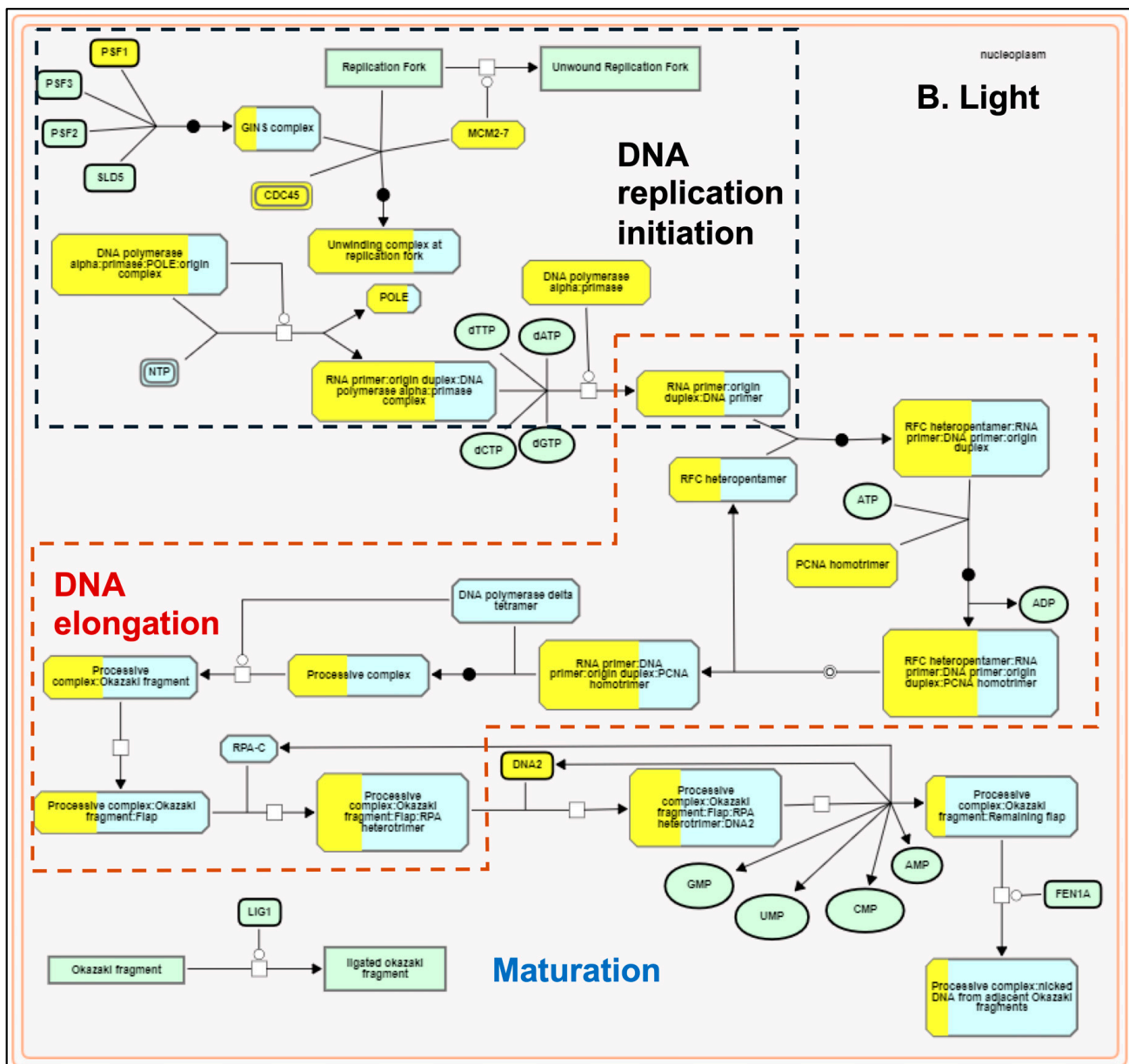
Figure 5. Plant Reactome pathway enrichment showing light-regulated RFC genes and reaction event coverage for the DNA biosynthesis pathway of the G1-to-S phase mitotic cell cycle. (A) shows enrichment in dark conditions and (B) shows enrichment in light conditions. Each reaction has several input and output entities and may be regulated or catalyzed by a protein and/or a protein complex. Solid arrows depict the directionality. The view also shows overlaps between the sub-pathways. The boxes with yellow-painted areas show the gene coverage (the number of genes mapped to the protein or protein complex entity participating in the respective reaction).
