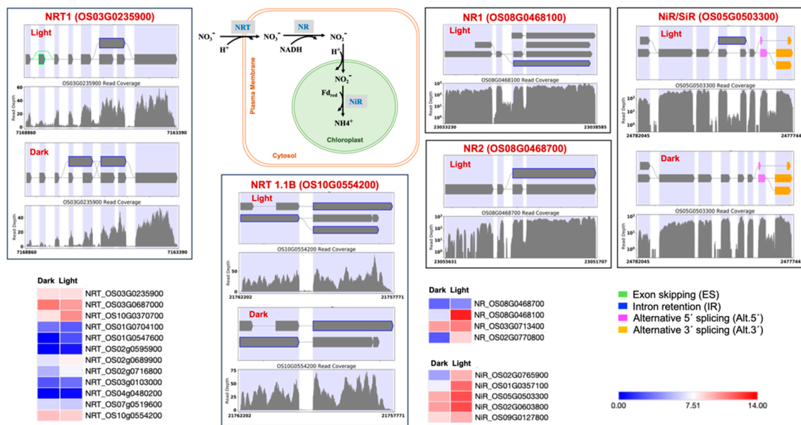
Figure 6. Splicing and expression pattern of nitrogen assimilation cycle genes under dark and light conditions. NRT: Nitrate transporter; NR: Nitrate reductase; NiR/SiR: Nitrite reductase/Sulfite reductase.
