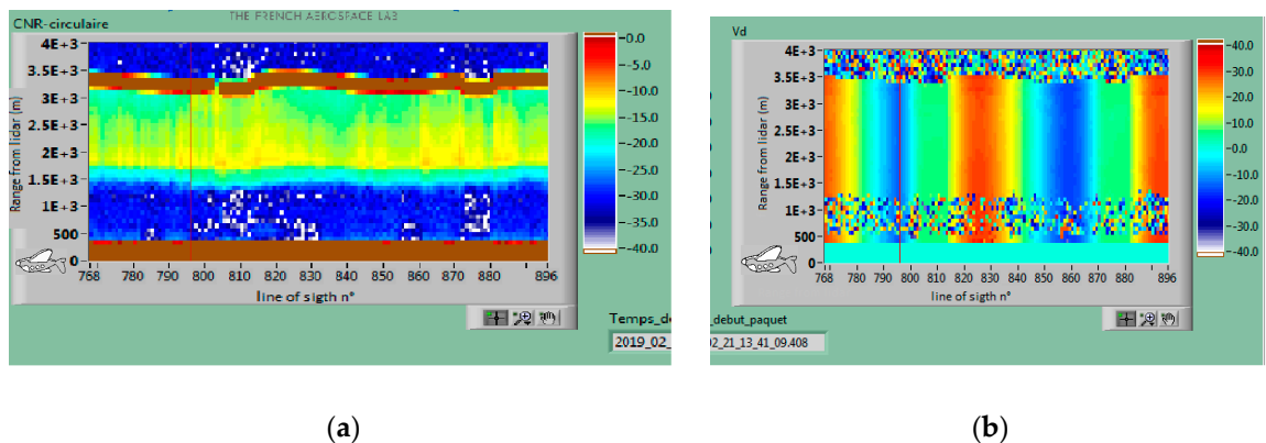
Figure 7. (a) Line of sight CNR real time display. (b) Line of sight velocity real time display for the conical scan. Range zero is the aircraft altitude while range 3500 m is the ground echo.
