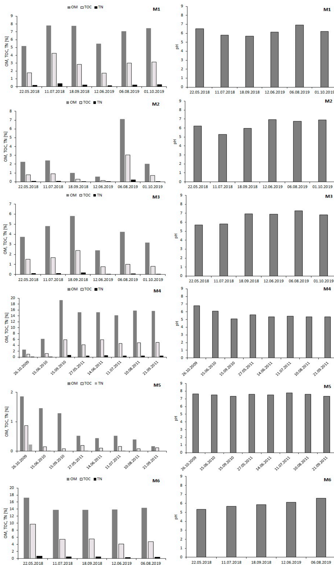
Figure S2. Organic matter (OM), total organic carbon (TOC), total nitrogen (TN) contents and pH in studied sediments in Maziarnia Reservoir.
