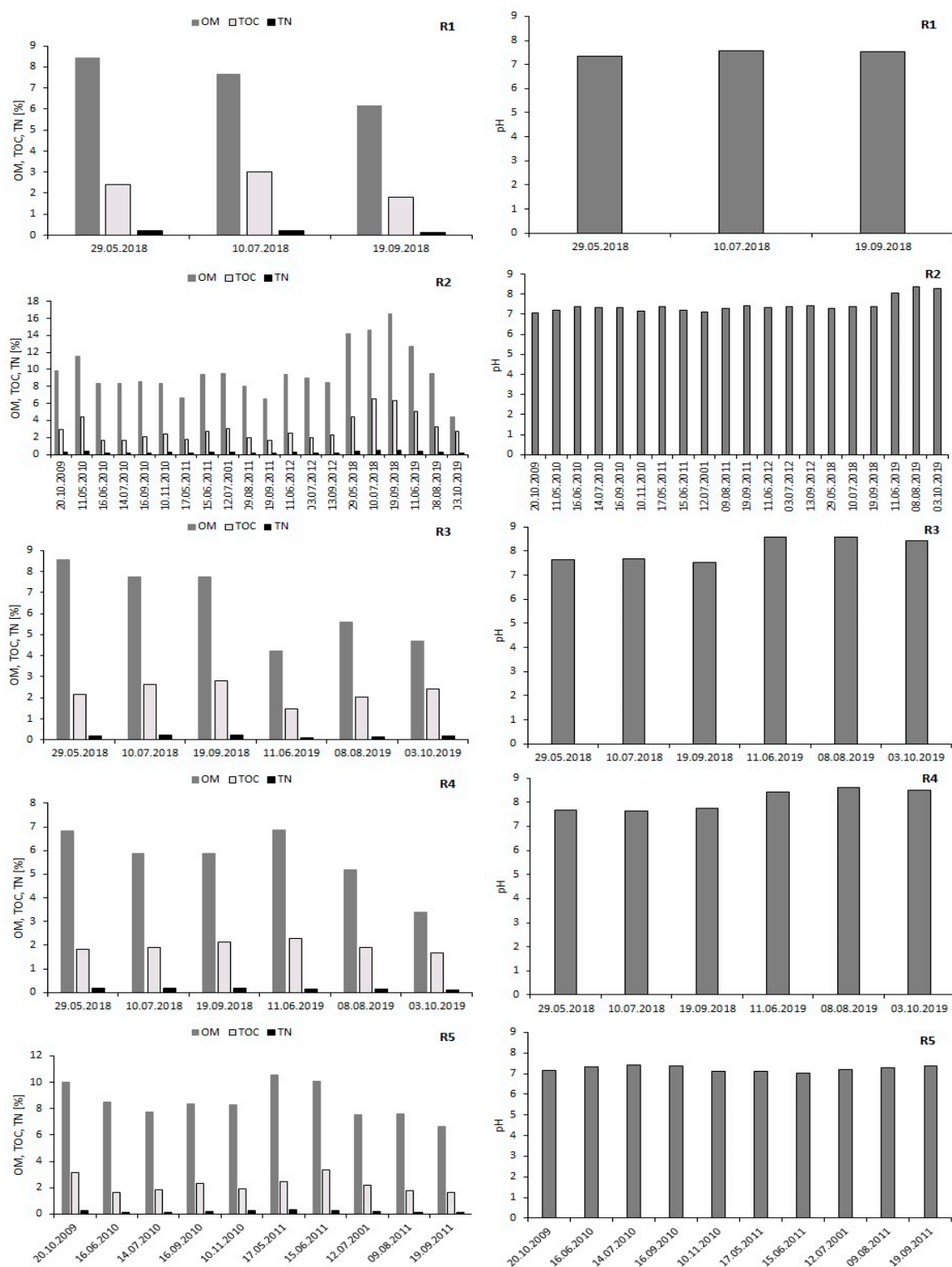
Figure S1. Organic matter (OM), total organic carbon (TOC), total nitrogen (TN) contents and pH in studied sediments in Rzeszów Reservoir.
