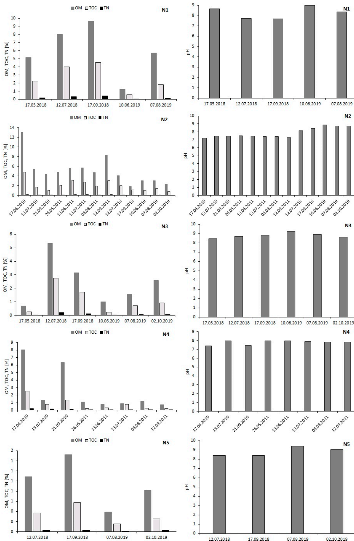
Figure S3. Organic matter (OM), total organic carbon (TOC), total nitrogen (TN) contents and pH in studied sediments in Nielisz Reservoir.
