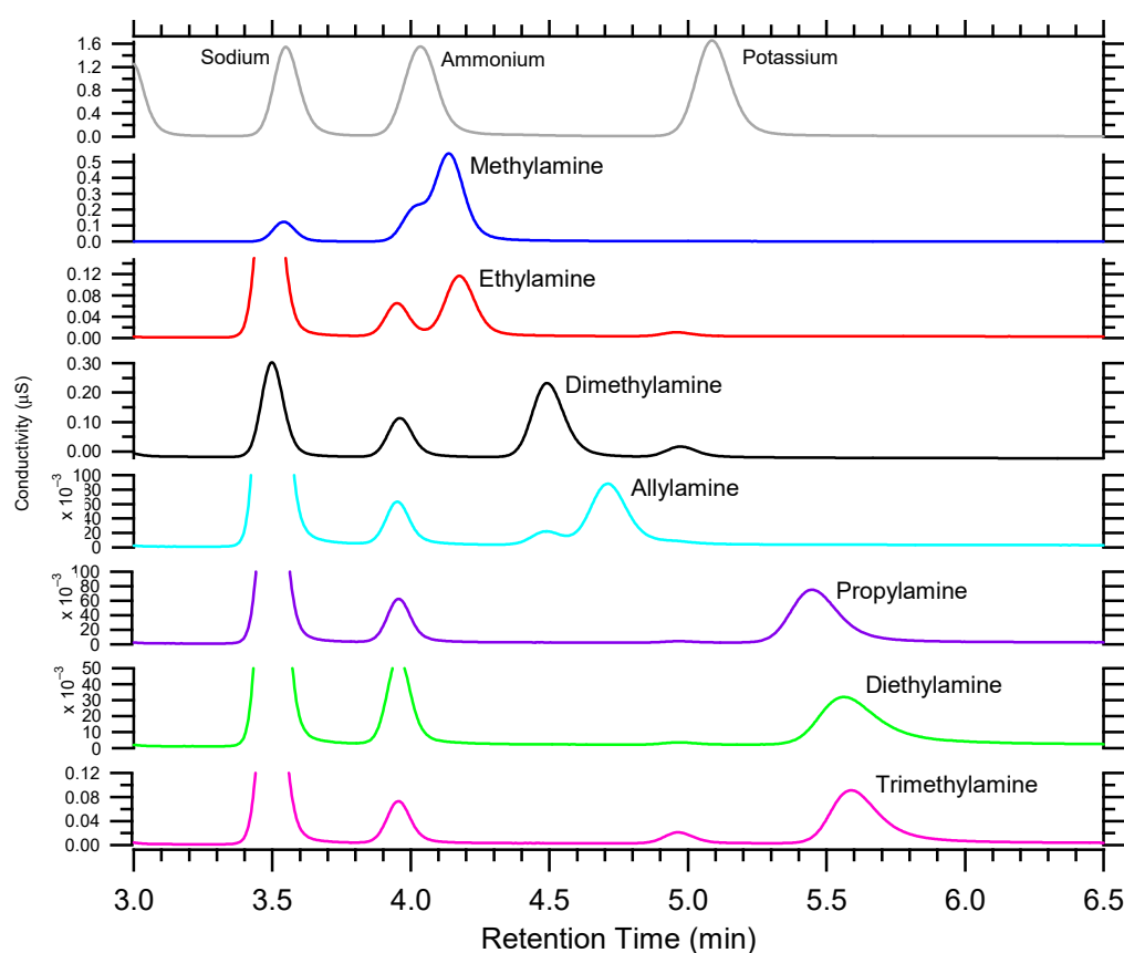
Figure 2. Chromatogram comparison of a cation and seven different amine calibration standards. The separation was performed on a Thermo Scientific Dionex IonPac CS-12A (3 × 150 mm) column using an isocratic method with an eluent of 20 mM methanesulfonic acid at a flowrate of 0.5 mL min -1 . Note only data from 3 to 6.5 min is being shown to illustrate the challenges with using this column to simultaneously measure the +1 inorganic cations and amines. It is observed that methylamine and ethylamine, as well as propylamine, diethylamine, and trimethylamine, overlap. In addition, there is overlap of ammonium with methylamine and ethylamine. Depending on the size of the ammonium peak, this could extend to dimethylamine and allylamine. Therefore, the ammonium concentration would be overestimated as these amines are being included in the integration of the ammonium peak. The same could be true for potassium, depending on the size of its peak, with propylamine, diethylamine, and trimethylamine.
