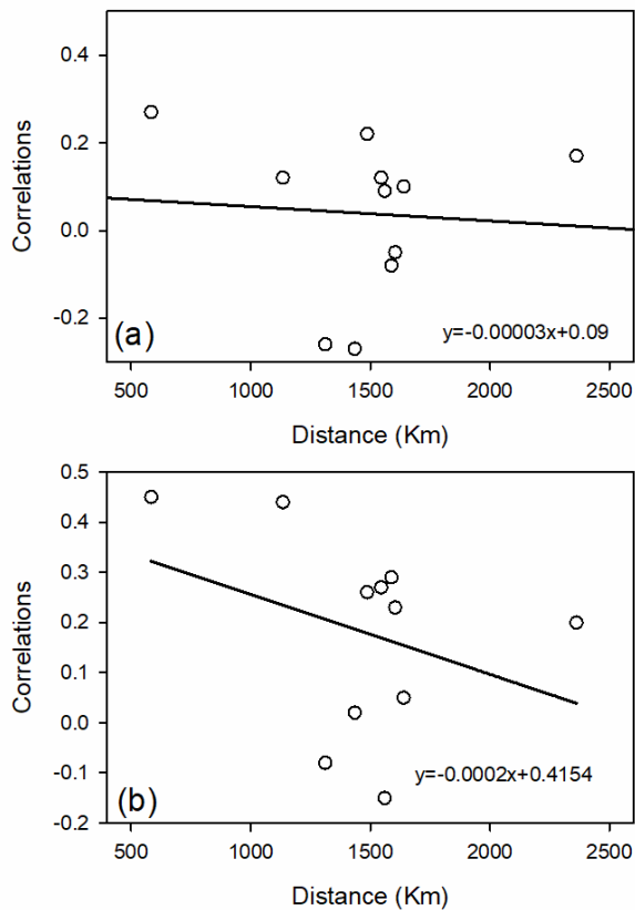
Figure S1 The linear regression of correlations between tree ring oxygen isotopes with summer (a) and winter (b) ice core oxygen isotope with that of distances between tree ring sampling site and ice core sites presented in Figure 3.
