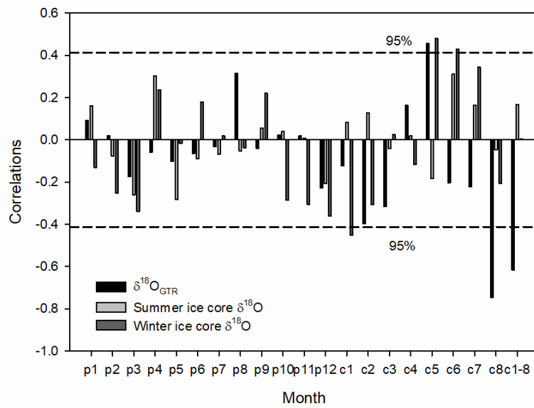
Figure S2 Correlations between tree ring oxygen isotope with NAO/AO during the period of 1950-1970. Numbers in x-axis represent the months of the year, and numbers with a “p” and “c” prefix indicate the previous year and current year, respectively.
