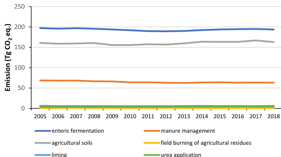
Figure 7. GHG emissions from agricultural sources in the EU in 2005–2018.
