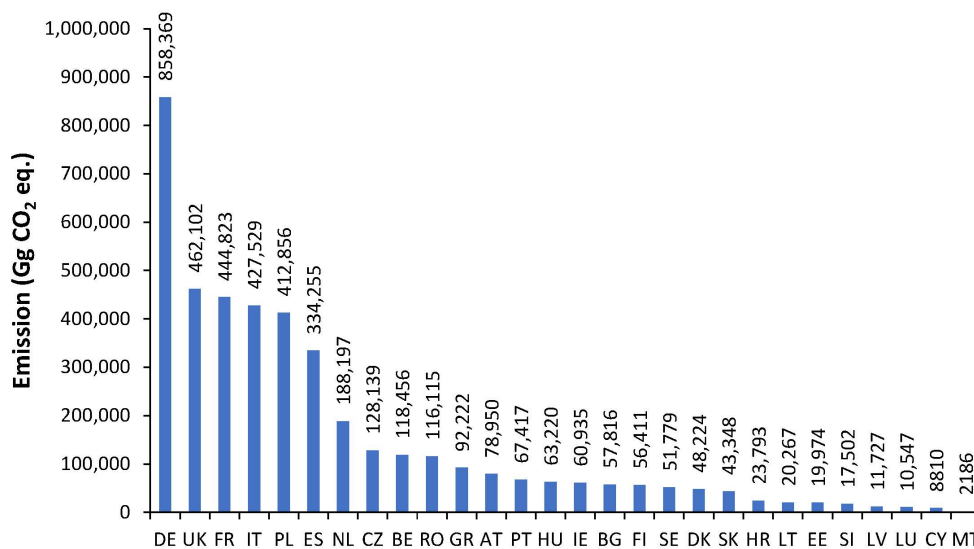
Figure 2. GHG emissions in the EU countries in 2018. Explanation: DE—Germany, UK—United Kingdom, FR—France, IT—Italy, PL—Poland, ES—Spain, NL—The Netherlands, CZ—Czech Republic, BE—Belgium, RO—Romania, GR—Greece, AT—Austria, PT—Portugal, HU—Hungary, IE—Ireland, BG—Bulgaria, FI—Finland, SE—Sweden, DK—Denmark, SK—Slovakia, HR—Croatia, LT—Lithuania, EE—Estonia, SI—Slovenia, LV—Latvia, LU—Luxembourg, CY—Cyprus, MT—Malta.
