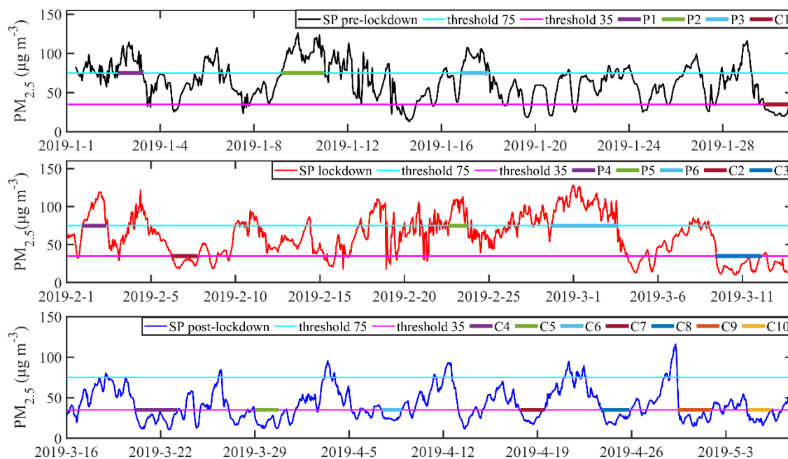
Figure S1. The time series of PM 2.5 during the same three study periods of pre-lockdown, lockdown, and post-lockdown in 2019 (SP19), along with the classification of pollution, moderate, and clean days. “threshold 75” represents the value is equal to 75. “threshold 35” represents the value is equal to 35. “P” represents pollution events and “C” represents clean events.
