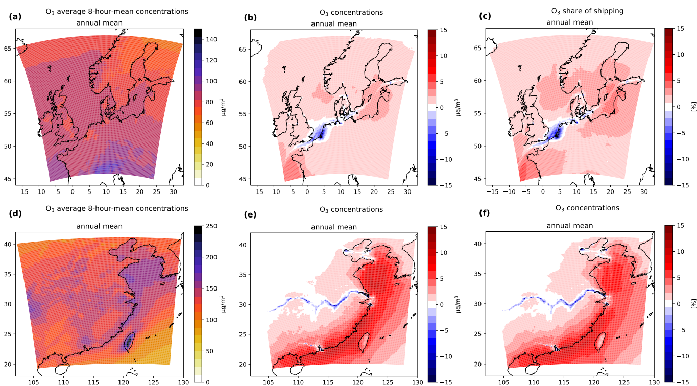
Figure 6. Annual averages of O_3 concentrations in the SC12NSBS domain for Europe (a–c) and in the CNC12 domain for China (d–f). Annual averages of 8-h max. O_3 concentrations [ \mu\text{g} \cdot \text{m}^{-3} ] from all emission sources are shown in (a,d), annual averages from shipping only in (b,e) and the share of O_3 concentrations from shipping on total O_3 concentrations [%] is shown in (c,f).
