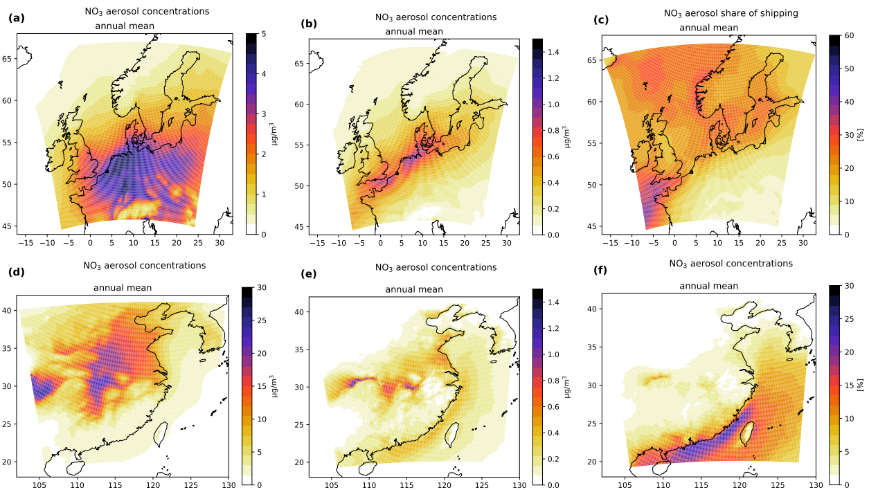
Figure 12. Annual averages of NO 3 concentrations in the SC12NSBS domain in Europe (a–c) and in the CNC12 domain in China (d–f). NO 3 concentrations [ \mu\text{g} \cdot \text{m}^{-3} ] from all emission sources are shown in (a,d); NO 3 concentrations only from shipping are shown in (b,e); the share of NO 3 concentrations from shipping in the NO 3 concentrations from all sources [%] is shown in (c,f).
