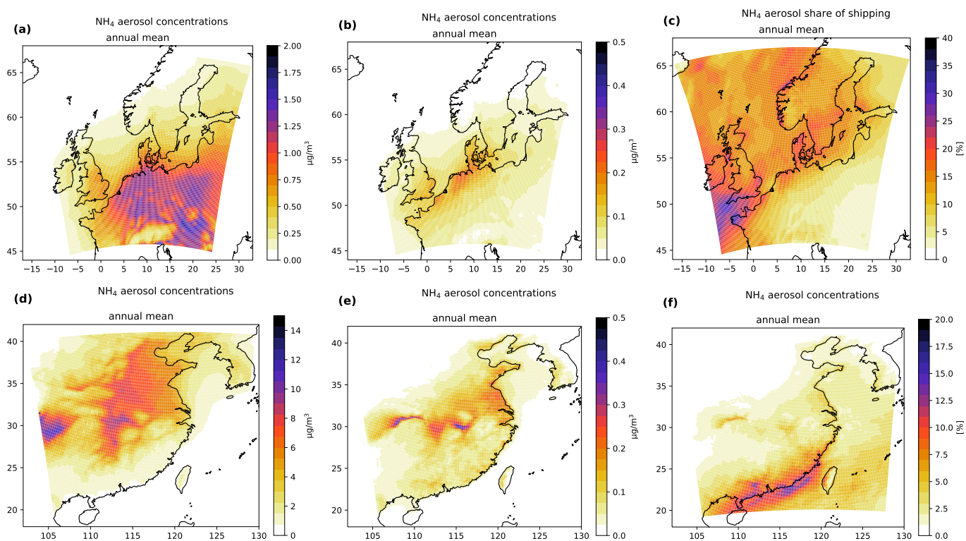
Figure 10. Annual averages of \text{NH}_4 concentrations in the SC12NSBS domain in Europe (a–c) and in the CNC12 domain in China (d–f). \text{NH}_4 concentrations [ \mu\text{g} \cdot \text{m}^{-3} ] from all emission sources are shown in (a,d); \text{NH}_4 concentrations only from shipping are shown in (b,e); the share of \text{NH}_4 concentrations from shipping in the \text{NH}_4 concentrations from all sources [%] is shown in (c,f).
