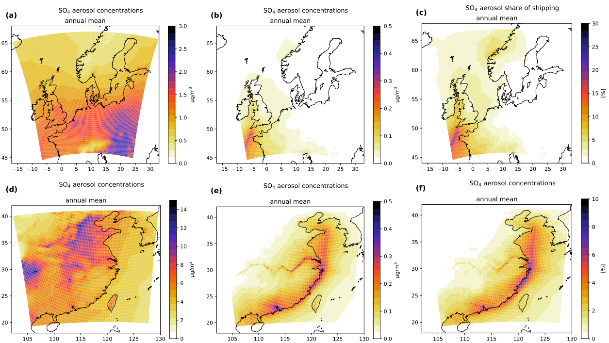
Figure 11. Annual averages of SO 4 concentrations in the SC12NSBS domain in Europe (a–c) and in the CNC12 domain in China (d–f). SO 4 concentrations [ \mu\text{g} \cdot \text{m}^{-3} ] from all emission sources are shown in (a,d); SO 4 concentrations only from shipping are shown in (b,e); the share of SO 4 concentrations from shipping in the SO 4 concentrations from all sources [%] is shown in (c) and (f).
