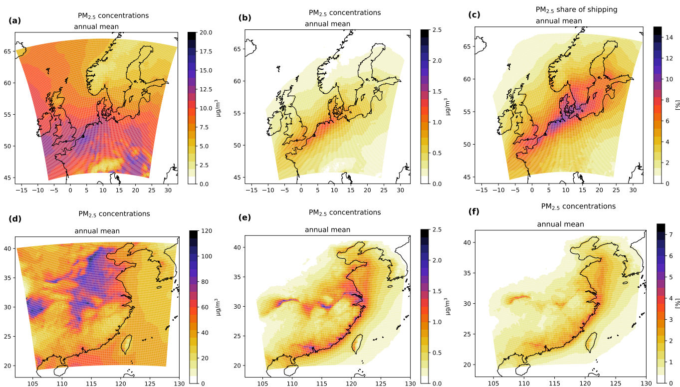
Figure 8. Annual averages of PM 2.5 concentrations in the SC12NSBS domain in Europe (a–c) and in the CNC12 domain in China (d–f). PM 2.5 concentrations [µg · m -3 ] from all emission sources are shown in (a,d); PM 2.5 concentrations only from shipping are shown in (b,e); the share of PM 2.5 concentrations from shipping in the PM 2.5 concentrations from all sources [%] is shown in (c,f).
