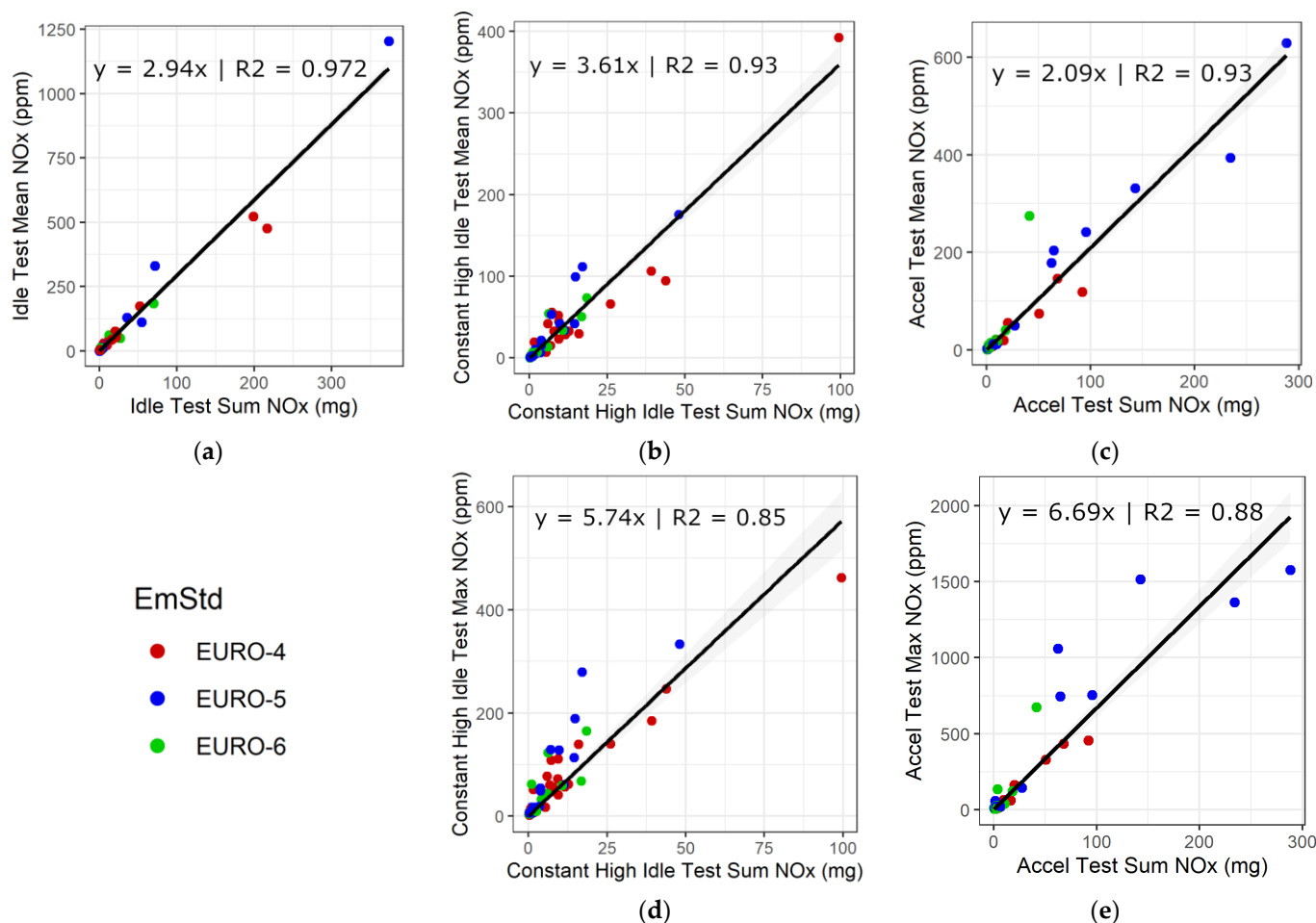
Figure 3. Petrol vehicle mean and maximum NOx concentration vs. total mass emissions over each test section: (a) idle test mean NOx; (b) high idle test mean NOx; (c) acceleration test mean NOx; (d) high idle test maximum NOx; (e) acceleration test maximum NOx.
