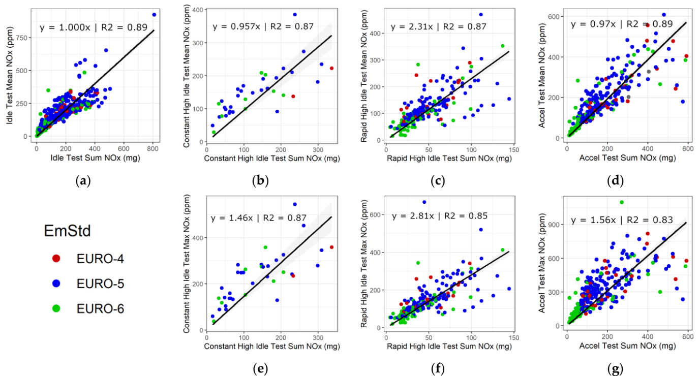
Figure 2. Diesel vehicle mean and maximum NO x concentration vs. total mass emissions over each test section: (a) idle test mean NO x ; (b) constant high idle test mean NO x ; (c) rapid high idle test mean NO x ; (d) acceleration test mean NO x ; (e) constant high idle test maximum NO x ; (f) rapid high idle test maximum NO x ; (g) acceleration test maximum NO x .
