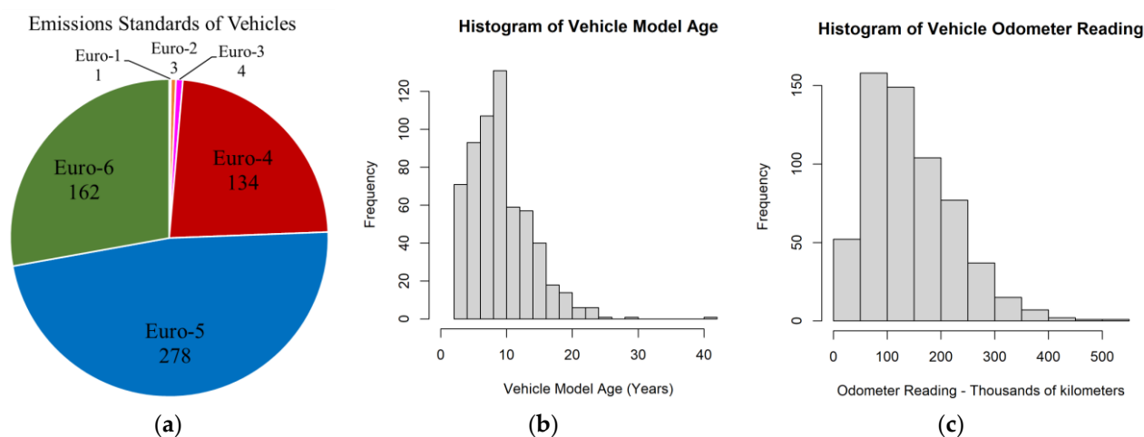
Figure 1. Fleet characteristics: (a) pie chart of vehicle emission standards (24 vehicles had pre-Euro or unknown Euro standard so are not represented here); (b) histogram of fleet model ages; (c) histogram of fleet odometer readings.
