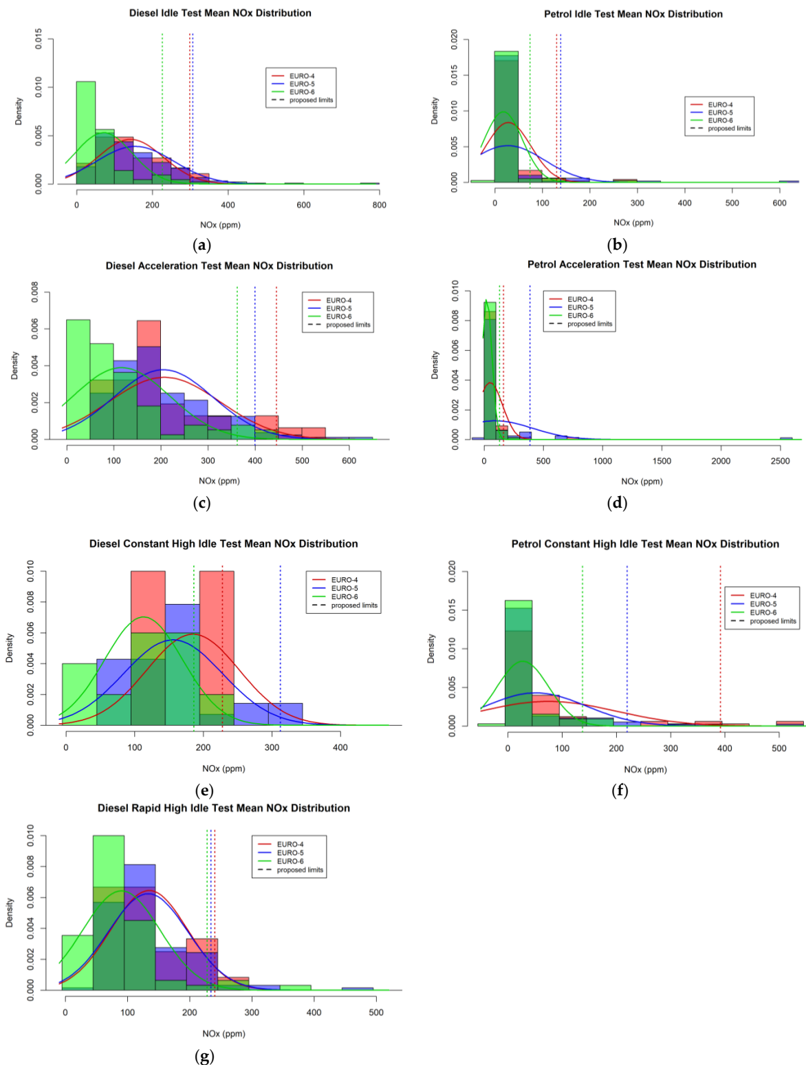
Figure 6. Diesel and petrol probability density distribution histograms for different test types, distributed into separate Euro standards (red bars—Euro 4, blue bars—Euro 5, green bars—Euro 6; colours are translucent to allow visualisation of all three Euro standards simultaneously), with 5% fail rate (i.e., 95th percentile) thresholds for each Euro standard marked by dashed lines: (a) diesel idle test; (b) petrol vehicle idle test; (c) diesel vehicle acceleration test; (d) petrol vehicle acceleration test; (e) diesel vehicle constant high idle test; (f) petrol vehicle constant high idle test; (g) diesel vehicle rapid high idle test.
