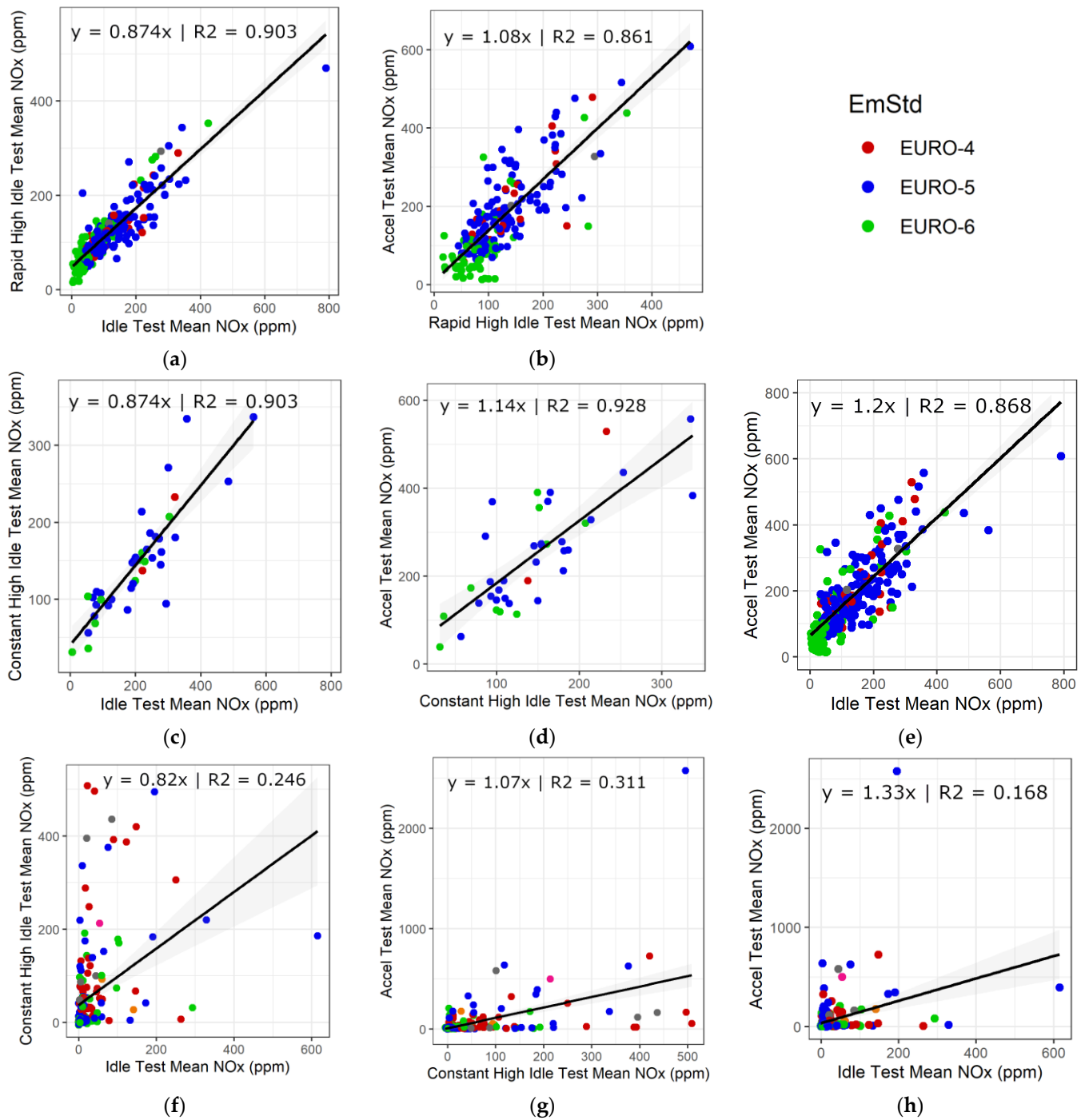
Figure 5. Diesel and petrol vehicle NOx concentrations compared between test types: (a) diesel vehicle rapid high idle test mean NOx versus idle test mean NOx; (b) diesel vehicle rapid high idle test mean NOx versus acceleration test mean NOx; (c) diesel vehicle constant high idle test mean NOx versus idle test mean NOx; (d) diesel vehicle constant high idle test mean NOx versus acceleration test mean NOx; (e) diesel vehicle acceleration test mean NOx versus idle test mean NOx; (f) petrol vehicle constant high idle test mean NOx versus mean idle test NOx; (g) petrol vehicle constant high idle test mean NOx versus acceleration test mean NOx; (h) petrol vehicle acceleration test mean NOx versus idle test mean NOx.
