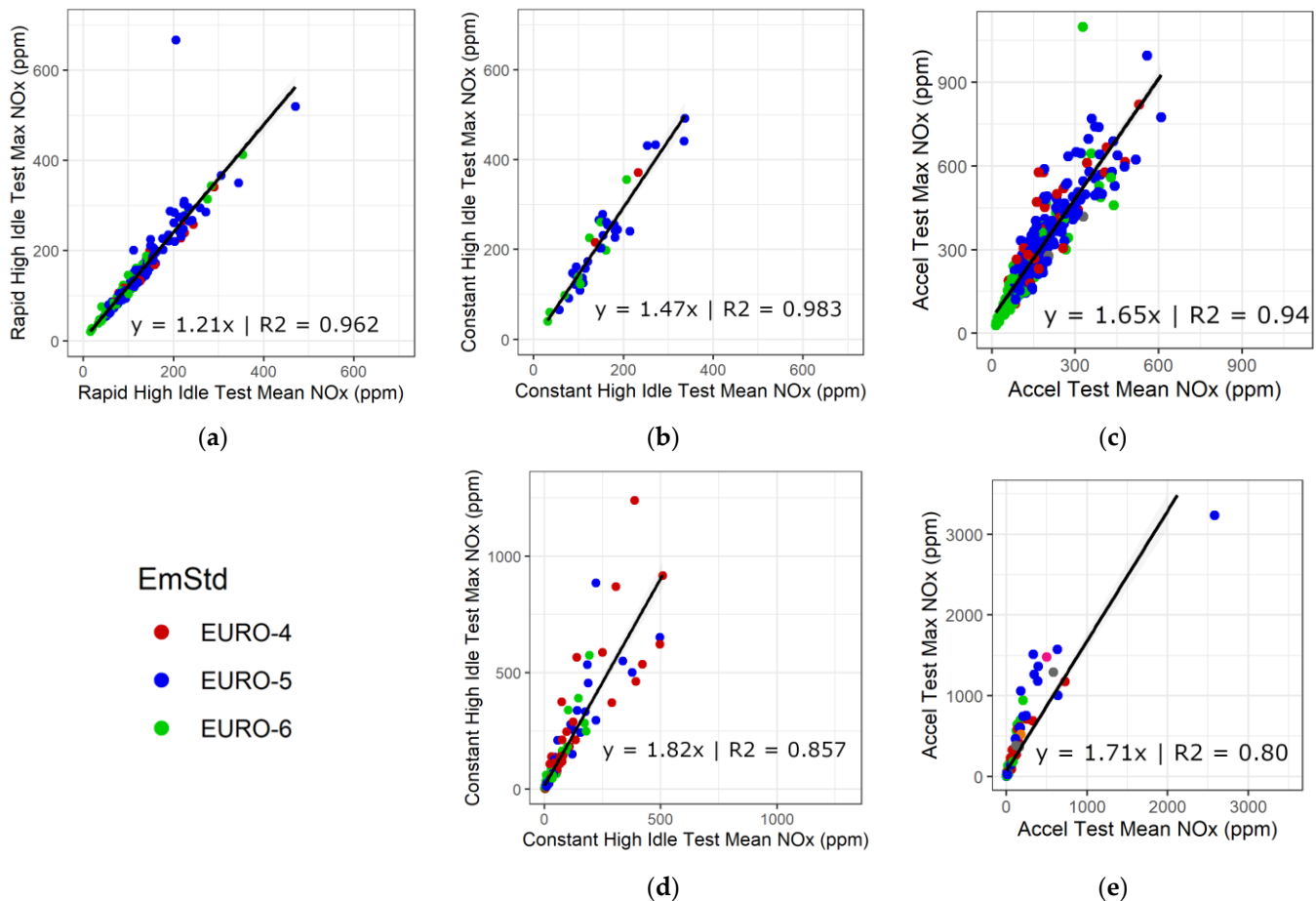
Figure 4. Petrol and diesel maximum NO x concentration versus mean NO x concentration for high idle and acceleration test sections: (a) diesel vehicle rapid high idle test; (b) diesel vehicle constant high idle test; (c) diesel vehicle acceleration test; (d) petrol vehicle constant high idle test; (e) petrol vehicle acceleration test.
