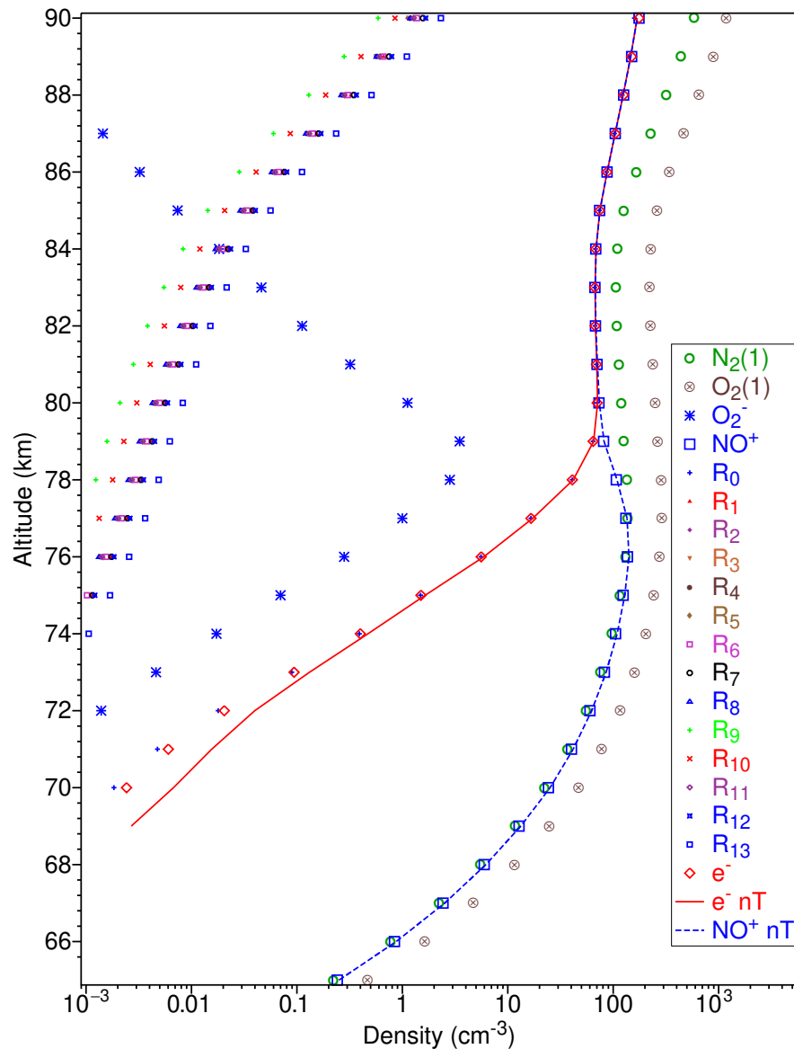
Figure 7. Calculated densities as a function of altitude: electron (—) and NO + (---) densities for the nT method; densities for electrons (◇), NO + (□), molecules and electron subranges as labelled for the EI method without elastic collisions included.
