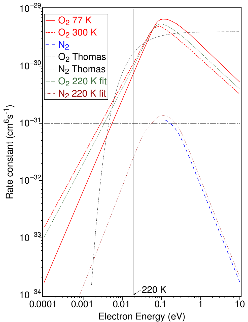
Figure 5. Rate constants ( \text{cm}^6 \text{s}^{-1} ) as a function of electron energy (eV) for attachment Reaction (R12) (labelled with “O 2 ”) measured [20] at 77 K (—) and 300 K (---), calculated for 220 K (—) and as given [13] for a Maxwellian distribution (-----). Similarly, for (R13) (labelled with “N 2 ”) measured [20] at 300 K (— — —), calculated for 220 K (---) and for a Maxwellian distribution [13] (-----).
