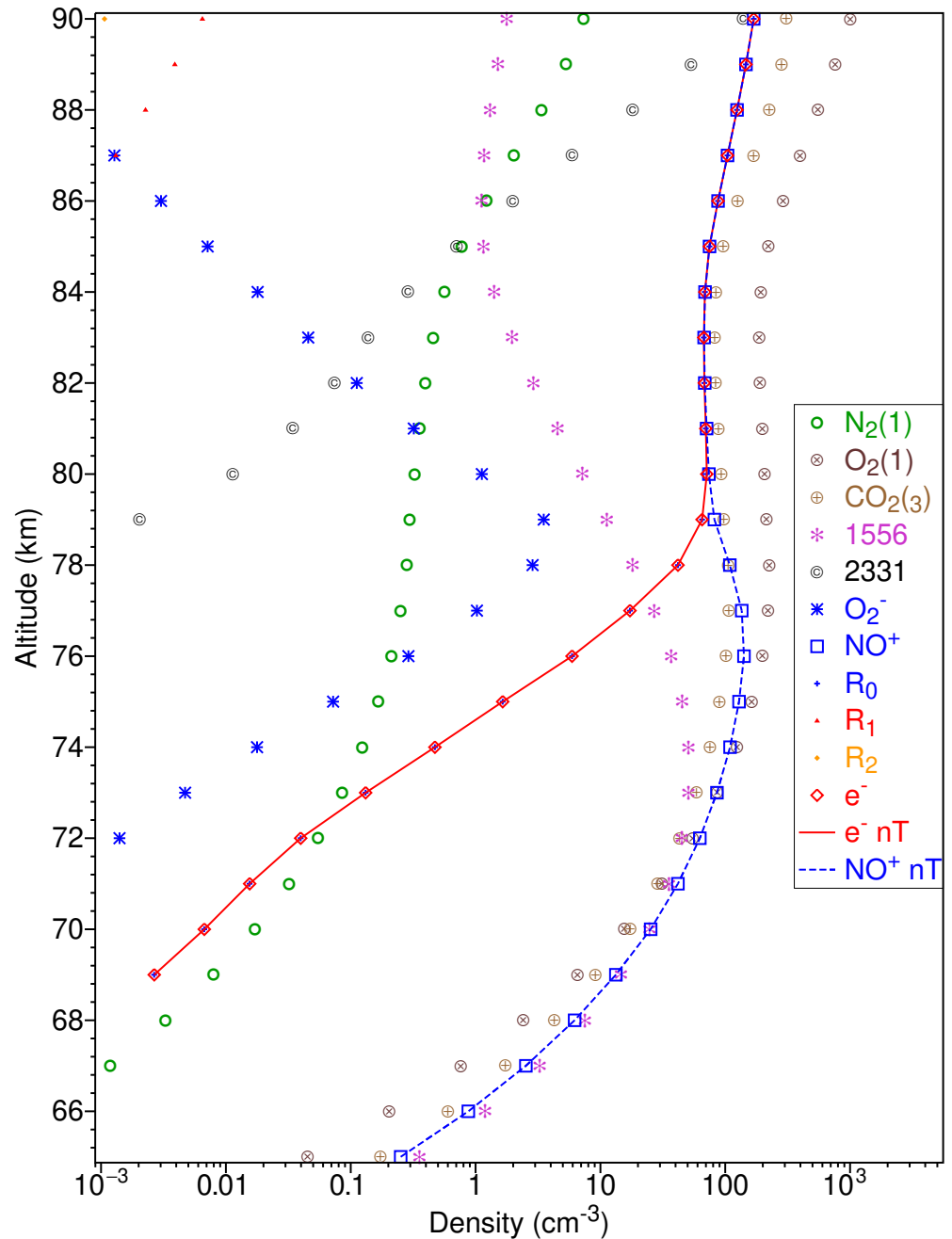
Figure 8. Calculated densities as a function of altitude: electron (—) and \text{NO}^+ (- - -) densities for the nT method; densities for electrons ( \diamond ), \text{NO}^+ ( \square ), molecules, electron subranges and emitted photons as labelled for the EI method with elastic scattering included.
