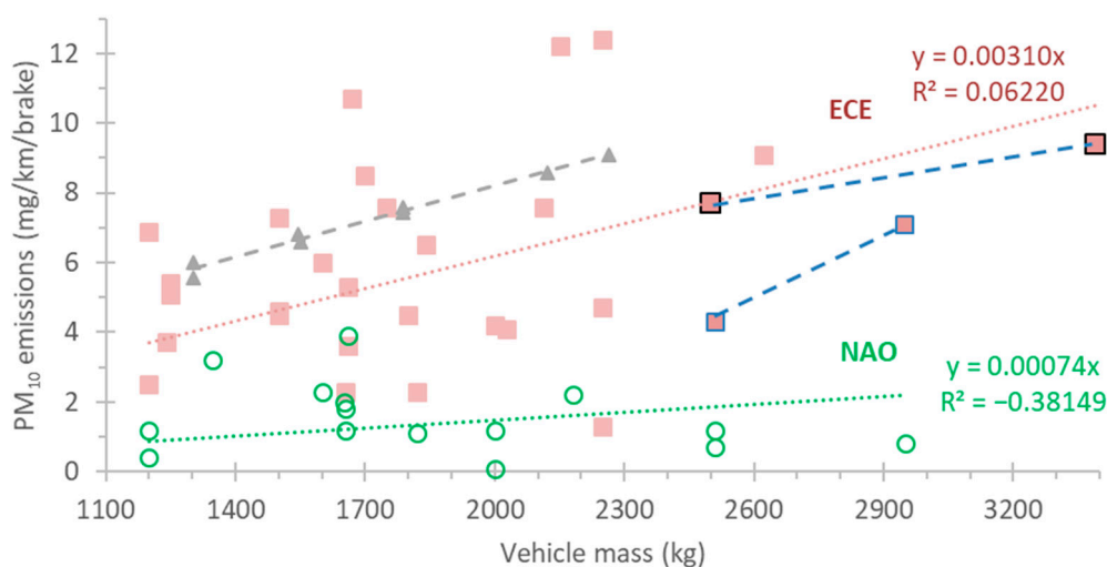
Figure 2. PM 10 emissions in function of vehicle mass for ECE (squares) and NAO (circles) pads and grey cast iron discs. Grey triangles and bigger squares with border are three dedicated studies that modified the vehicle mass and the dashed lines show their trendline assuming linear correlation for each study. The dotted lines give the correlation line of the ECE and NAO brakes of Table 2.
