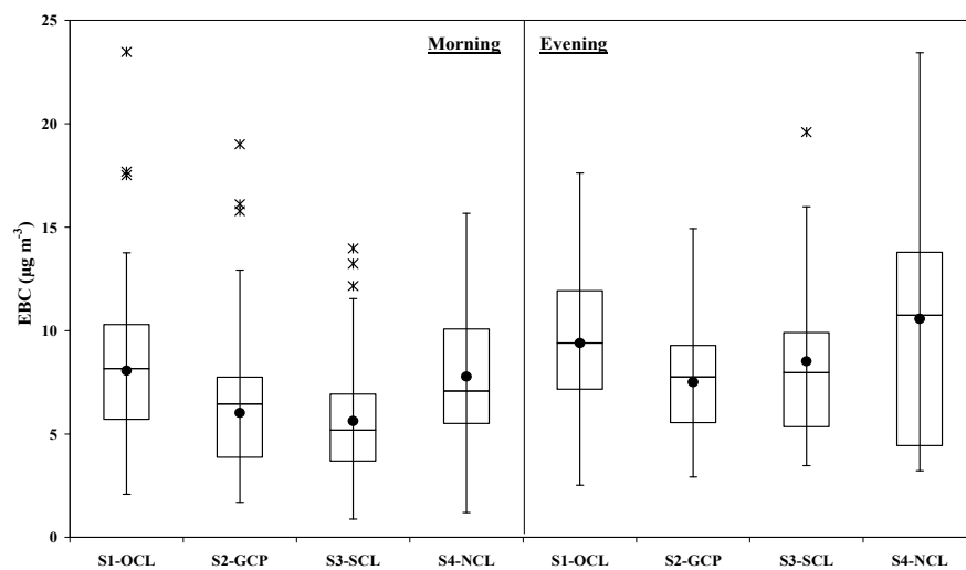
Figure 4. Box-plots of 1-min concentration data for EBC in the cold season (mean values: dots; min-max range: whiskers; median and interquartile range: boxes).
