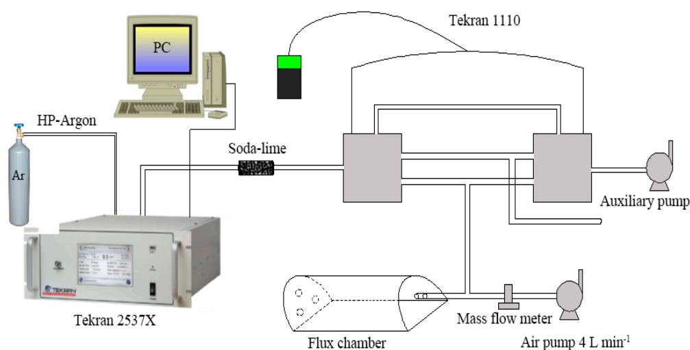
Figure S1. A diagram of GEM fluxes between soil-air interface.
