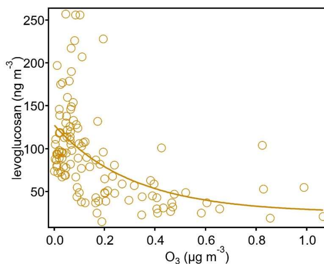
Figure S1. The negative correlation between levoglucosan ( \text{ng}/\text{m}^3 ) and \text{O}_3 ( \mu\text{g}/\text{m}^3 ).
