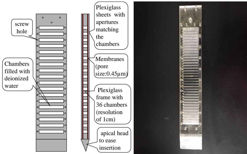
Figure S2. Schematic and physical photograph of Peeper.
