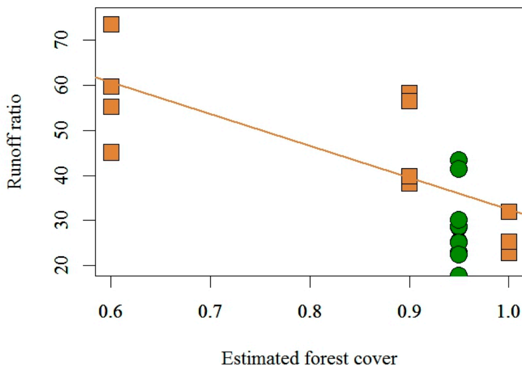
Figure S1. Comparison of runoff ratio versus percent vegetation cover.
