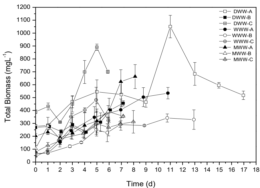
Figure S3: Profile of suspended and total biomass production through time using different dilution ratios (A, B, C) of wastewater as growth medium [DWW: dairy wastewater, WWW: winery wastewater, MWW: mixed (winery and raisin) wastewater].
