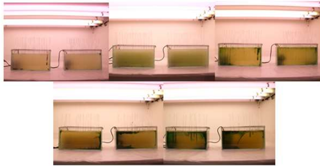
Figure S1: Photographs of the experimental PBRs showing the gradual increase of microbial biomass in attached culture systems with dairy wastewater as growth substrate (1 st to 7 th day of culture).
