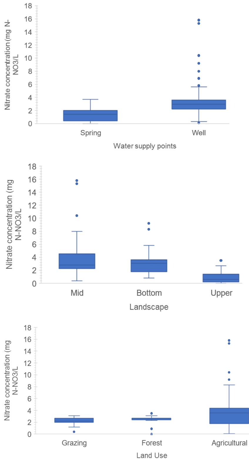
Figure S1. Boxplots of the nitrate concentrations in groundwater measured in developed springs and wells at three hillslope position and land use in the waterpoint drinking area in South Gondar Zone from December 2013 to June 2014
