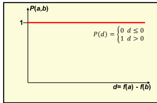
Figure 2. Usual criterion (Type I) preference function.
