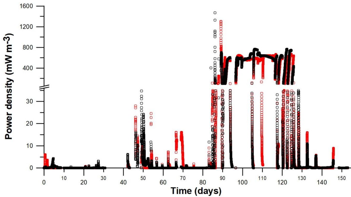
Figure S1. Performance CW-MFC during the four periods (152 days of operation). An increase in power density is observed from day 83 to day 124, when the anode potential was poised at -150 mV vs Ag/AgCl. Each curve color represents the two tested CW-MFC reactors (duplicates).
