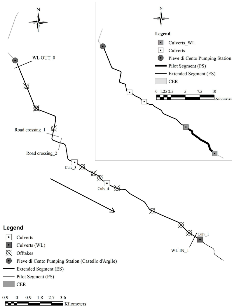
Figure 5. The scheme of ES: The 12 irrigation offtakes, the three culverts under passing the Idice River (Culv_1), the Navile Canal (Culv_3), and the Savena River (Culv_4), the two water gauges (WL OUT_0 and WL IN_1) at the OUT of the pumping station Pieve di Cento and at the IN of Culv_1, the two road crossings.
